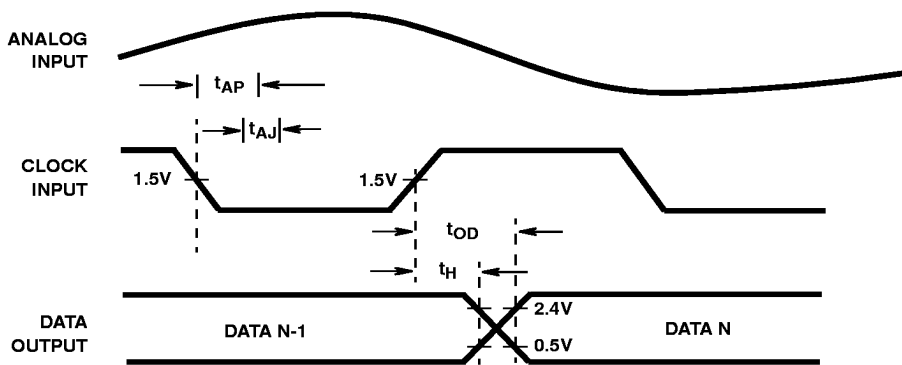
FIGURE 2. INPUT-TO OUTPUT TIMING
