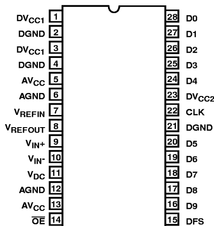
HI5767 (SOIC, SSOP) TOP VIEW
