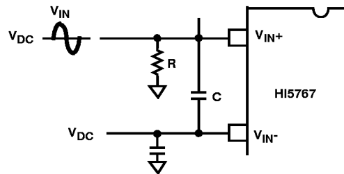
FIGURE 7. DC COUPLED SINGLE ENDED INPUT
