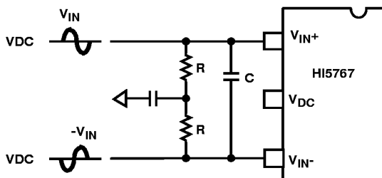
FIGURE 5. DC COUPLED DIFFERENTIAL INPUT
