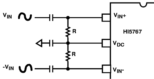
FIGURE 4. AC COUPLED DIFFERENTIAL INPUT
