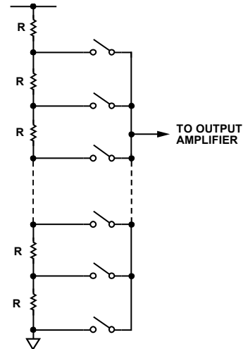
Figure 51. Resistor String
