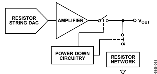
Figure 56. Output Stage During Power-Down
