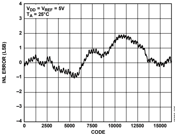
Figure 5. INL AD5644R, External Reference
