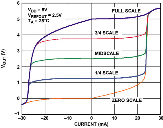
Figure 34. AD56x4R-5 Source and Sink Capability
