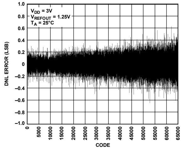
Figure 19. DNL AD5664R-3, Internal Reference
