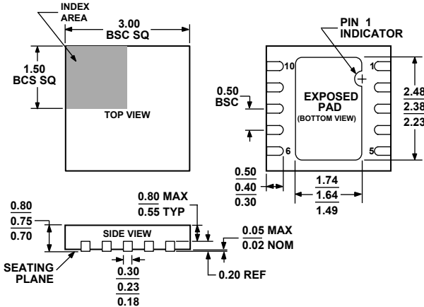
Figure 64. 10-Lead Lead Frame Chip Scale Package [LFCSP_WD] 3 mm × 3 mm Body, Very Very Thin, Dual Lead (CP-10-9) Dimensions shown in millimeters
