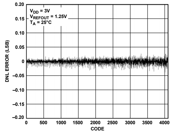
Figure 21. DNL AD5624R-3, Internal Reference
