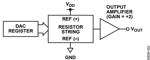
Figure 50. DAC Architecture
