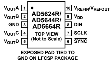
Figure 3. Pin Configuration
