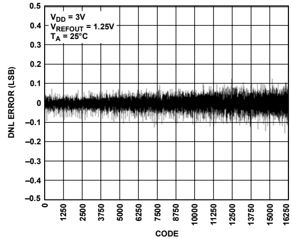
Figure 20. DNL AD5644R-3, Internal Reference
