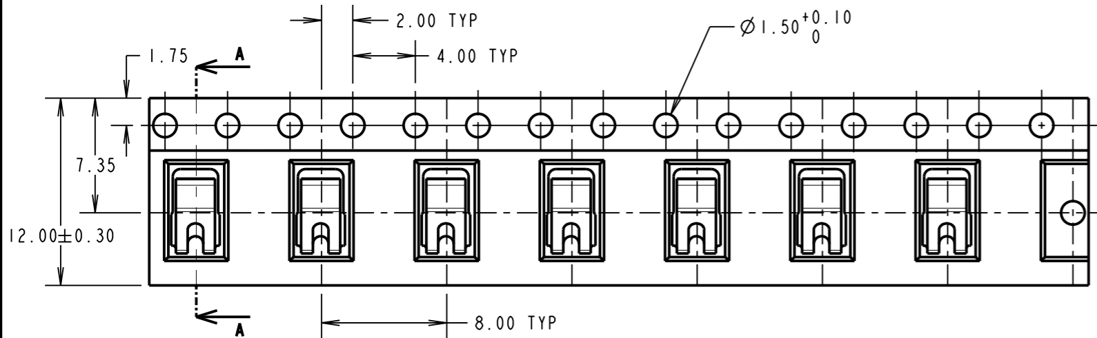
TAPE DIMENSIONS
