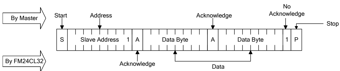
Figure 8. Sequential Read
