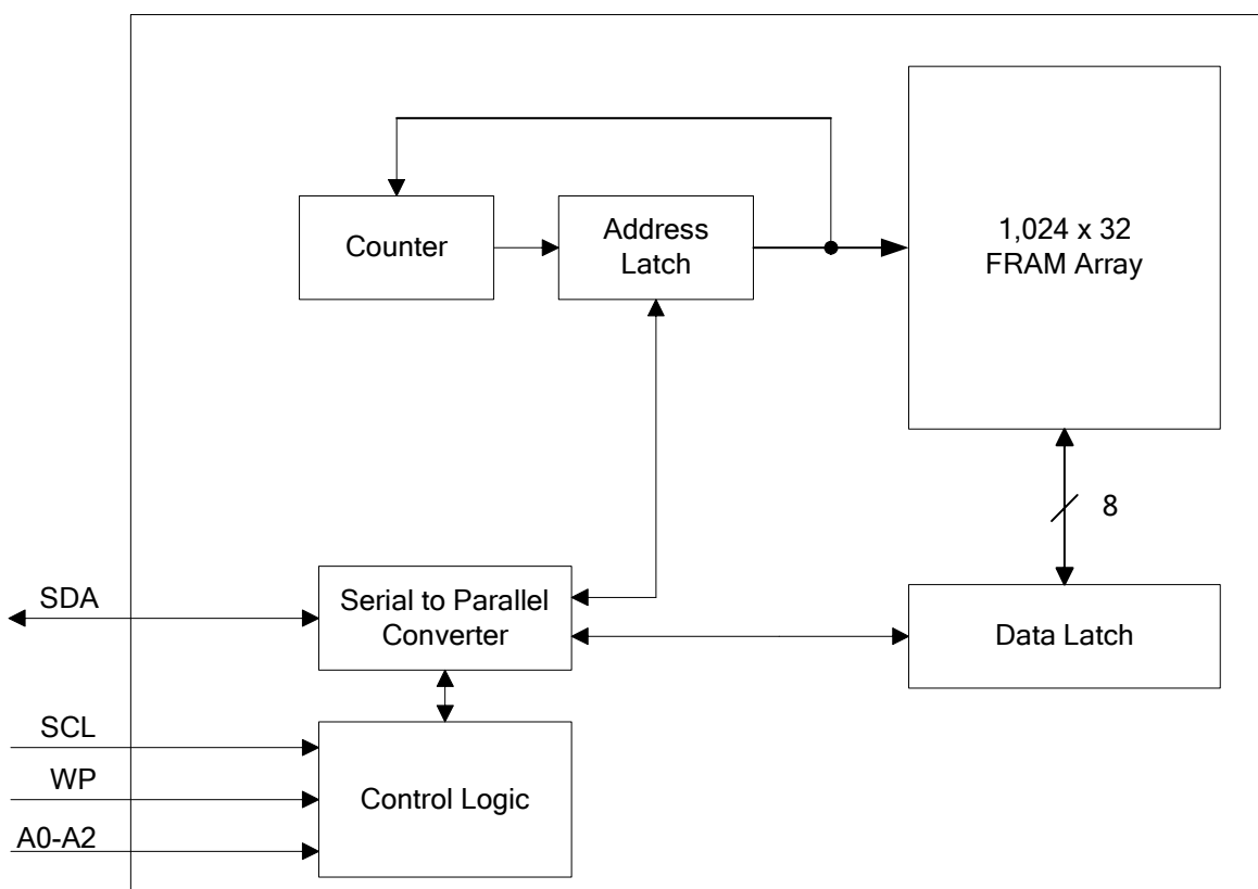
Figure 1. FM24CL32 Block Diagram
