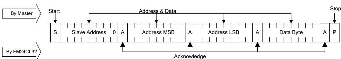
Figure 5. Single Byte Write
