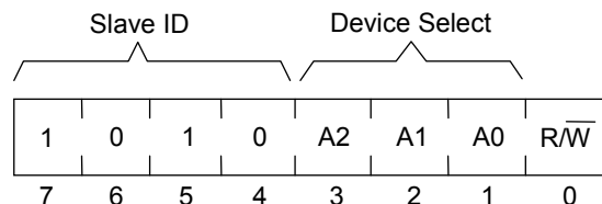
Figure 4. Slave Address
