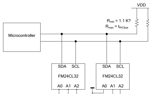
Figure 2. Typical System Configuration
