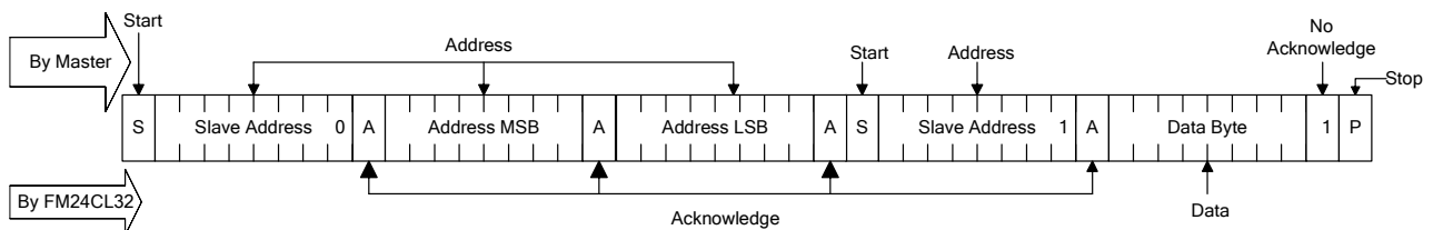
Figure 9. Selective (Random) Read
