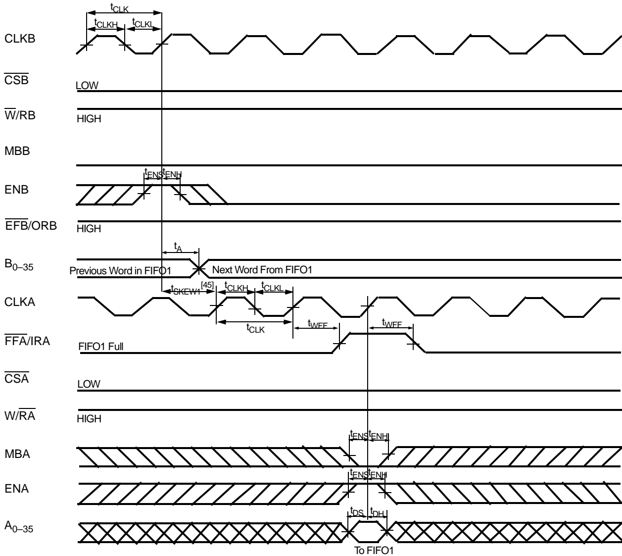
IRA Flag Timing and First Available Write when FIFO1 is Full (FWFT Mode) [42]
