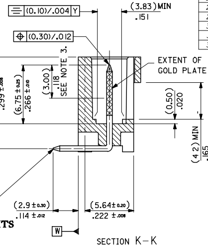
SECTION K-K
