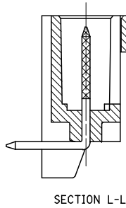
SECTION L-L
