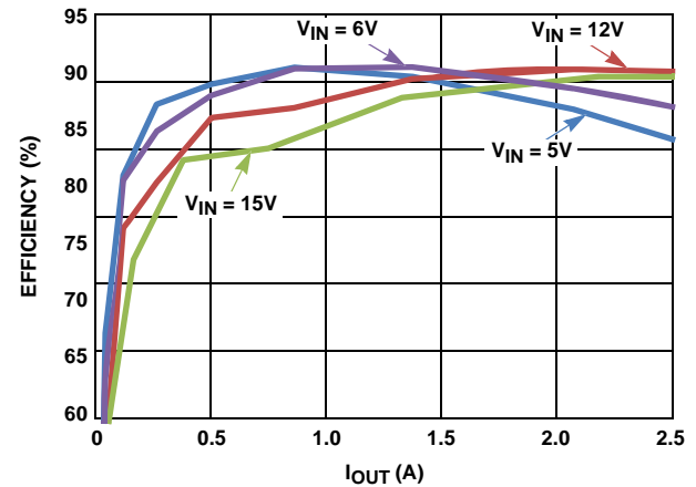
FIGURE 4. ISL85033-12VEVAL3Z EFFICIENCY: V_{OUT} = -5V
