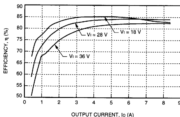
Figure 4. Typical FC100B Efficiency vs. Output Current at Room Temperature
