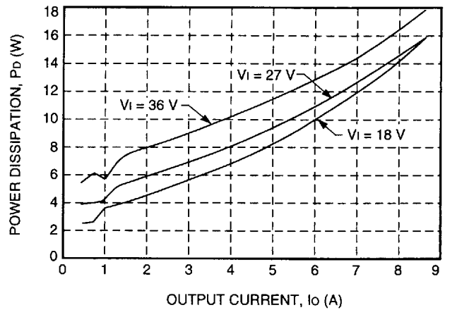
Figure 22. Power Dissipation as Heat vs. Output Current
