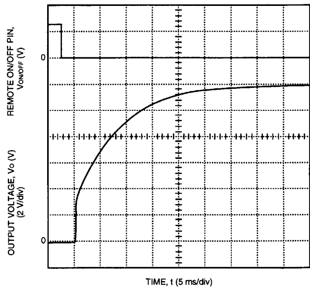
Figure 8. Typical FC100B Start-Up Transient at Room Temperature, 28 V Input, and 8.3 A Output
