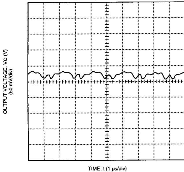
Figure 5. Typical FC100B Output Ripple Voltage at Room Temperature, 28 V Input, and 8.3 A Output
