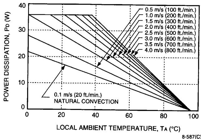
Figure 19. Power Derating vs. Local Ambient Temperature and Air Velocity
