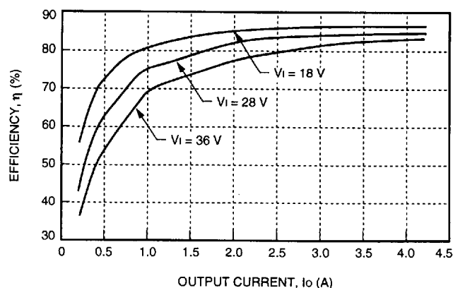
Figure 3. Typical FC050B Efficiency vs. Output Current at Room Temperature
