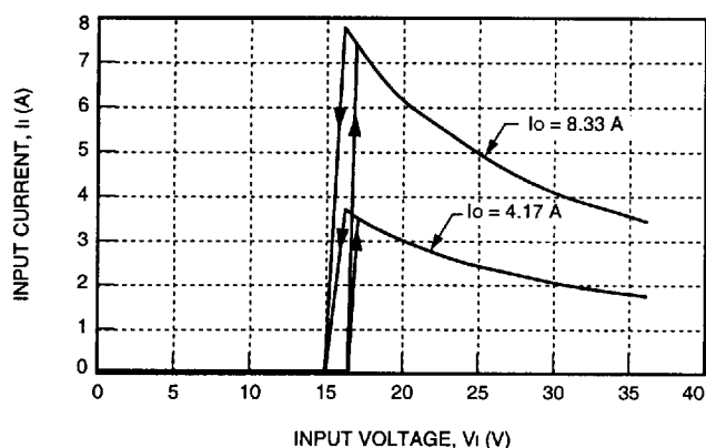
Figure 1. Typical FC100B Input Characteristics at Room Temperature
