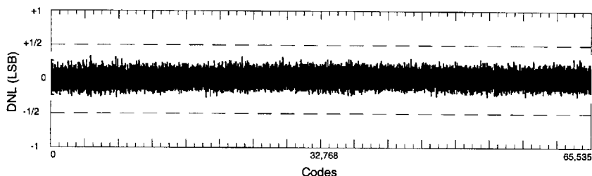
Figure 4. CS5509 Differential Nonlinearity plot.
