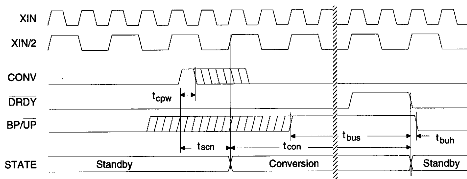
Figure 2. Conversion Timing (Not to Scale)
