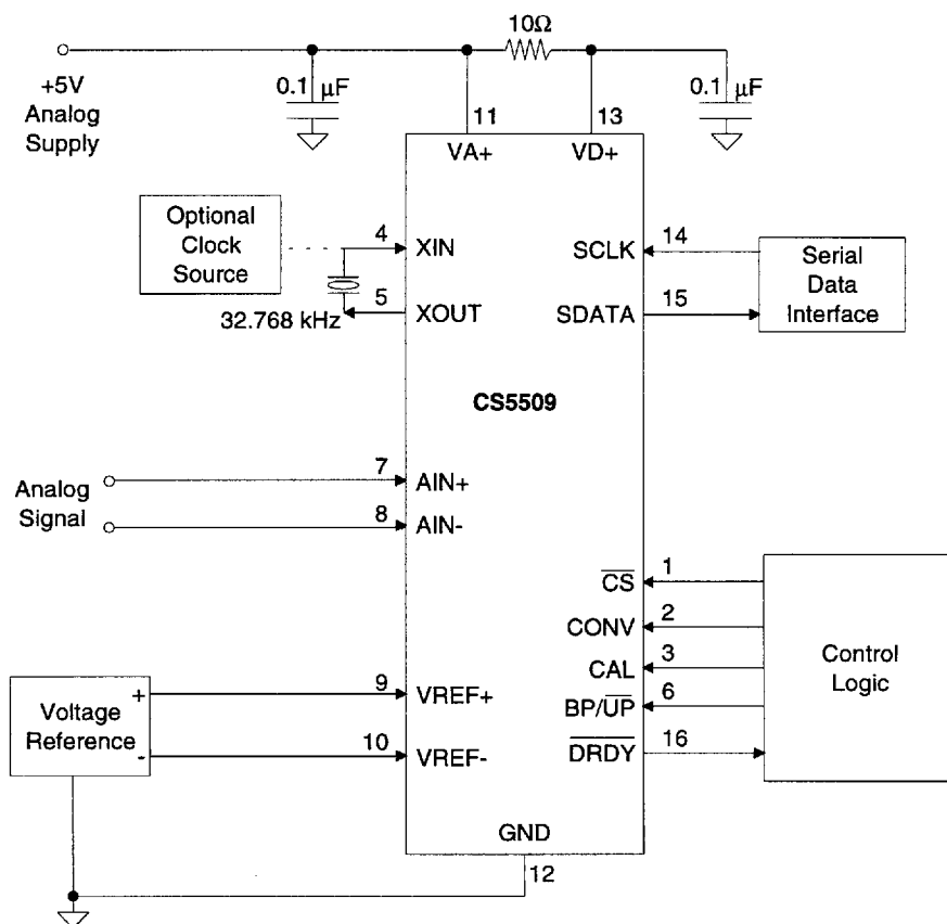
Figure 9a. System Connection Diagram Using a Single Supply
