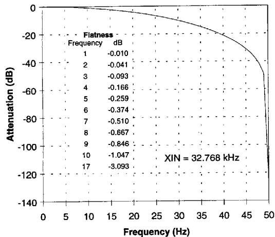
Figure 7. Filter Magnitude Plot to 50 Hz
