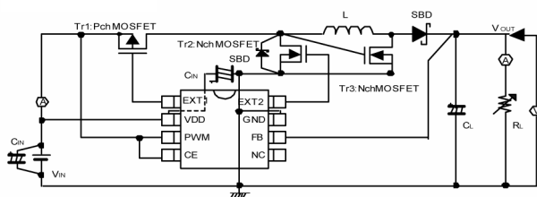
Circuit ③
