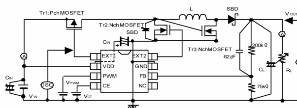
Circuit ④
