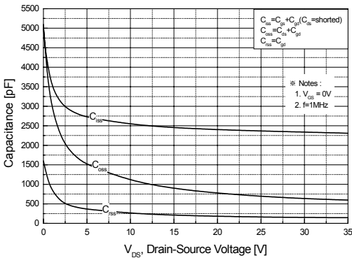
Fig 5. Capacitance Characteristics
