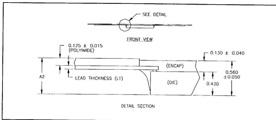
Figure 18. One TCP Site (Cross-Sectional Detail)
