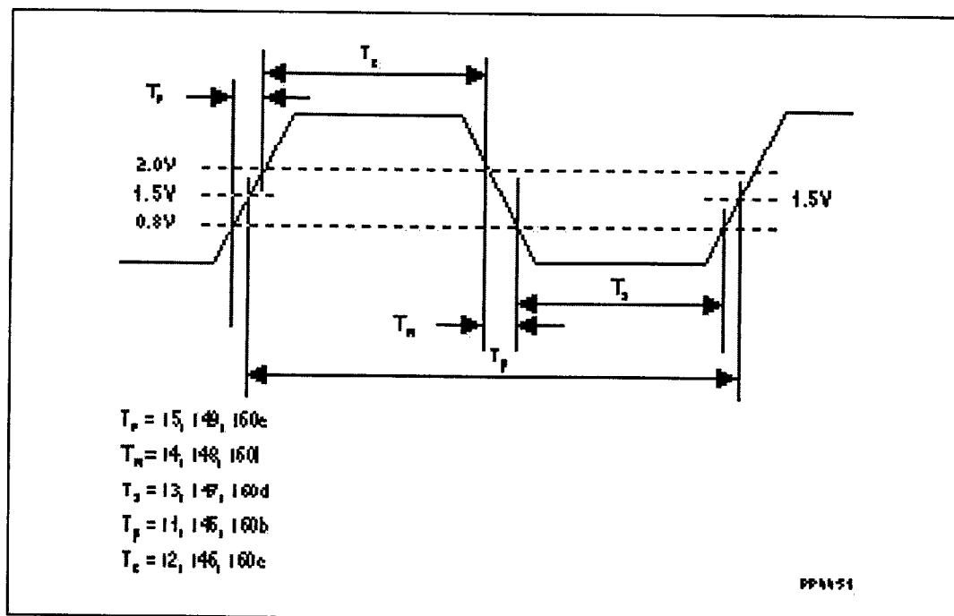
Figure 3. Clock Waveform
