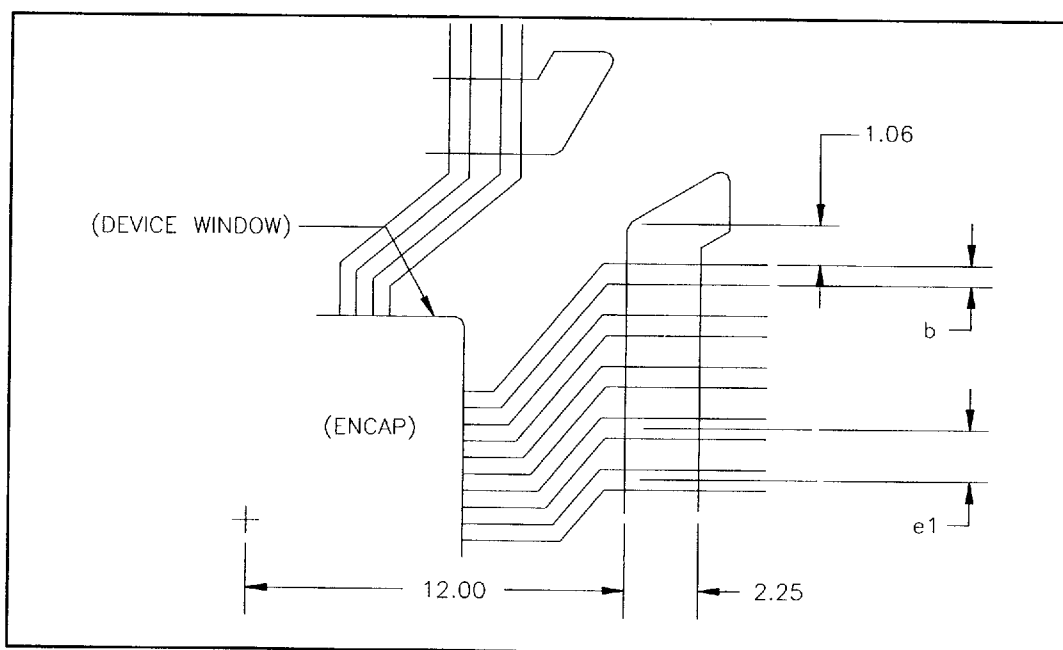
Figure 19. Outer Lead Bond (OLB) Window Detail
