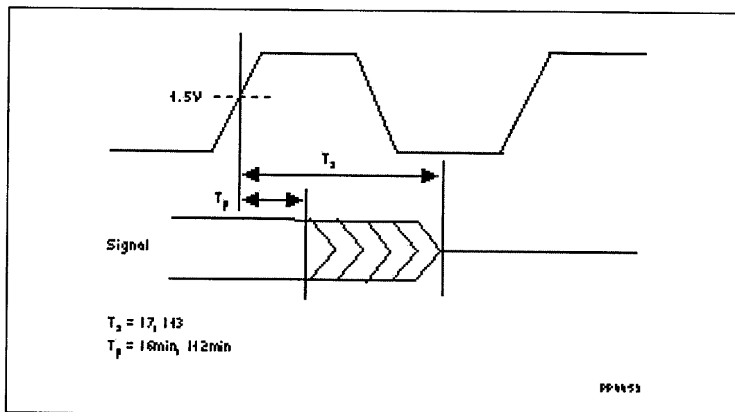
Figure 5. Float Delay Timings
