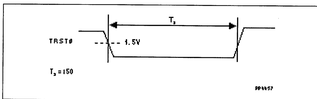
Figure 9. Test Reset Timings
