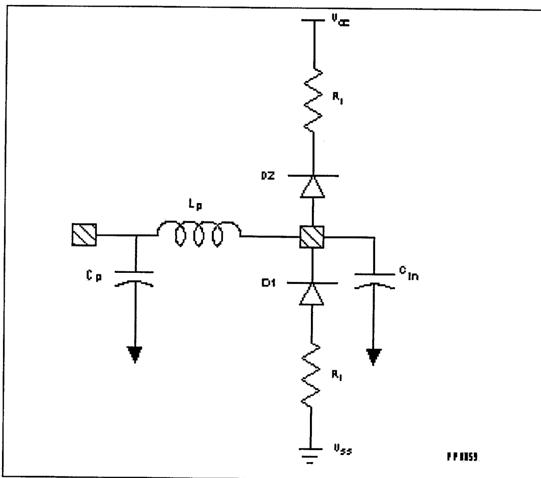
Figure 10. Input Buffer Model, Except Special Group
