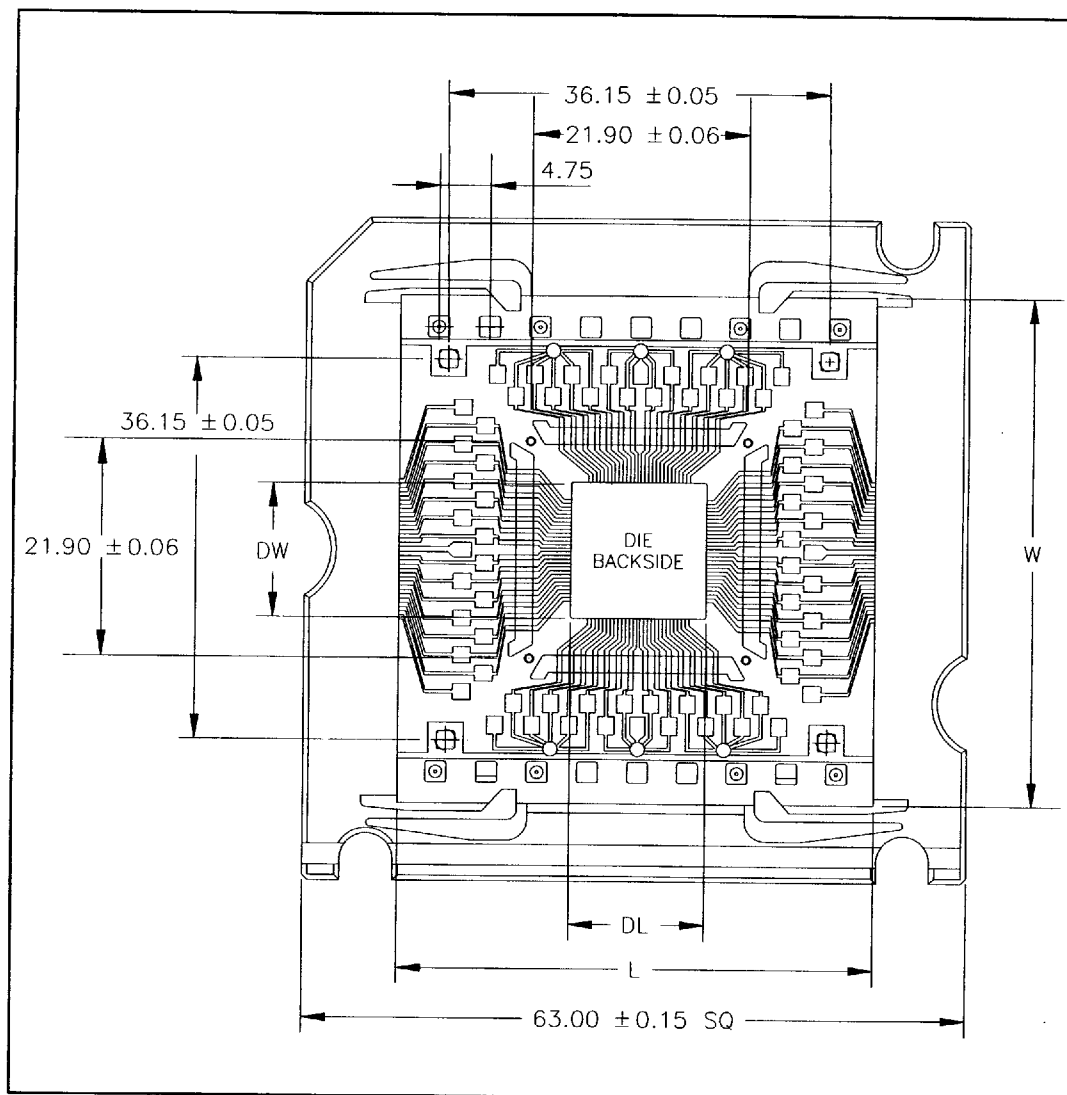
Figure 16. One TCP Site in Carrier (Bottom View of Die)
