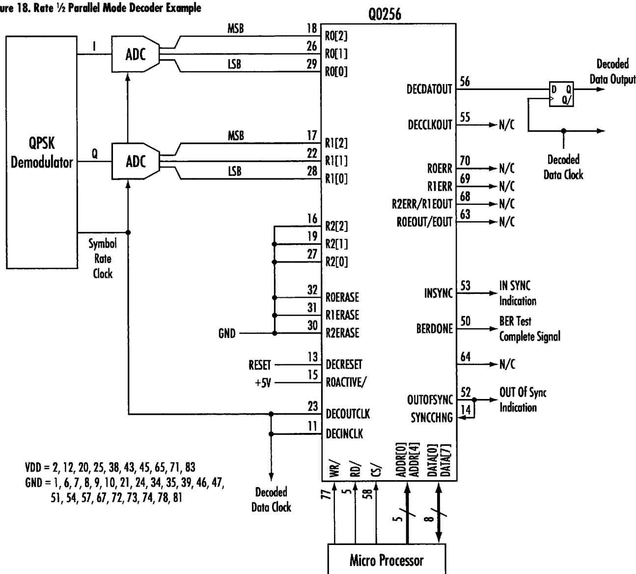
Figure 18. Rate 1/2 Parallel Mode Decoder Example
