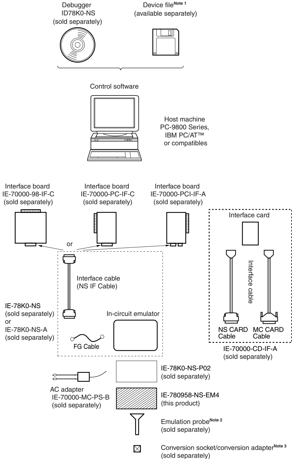
Figure 1-1. System Configuration
