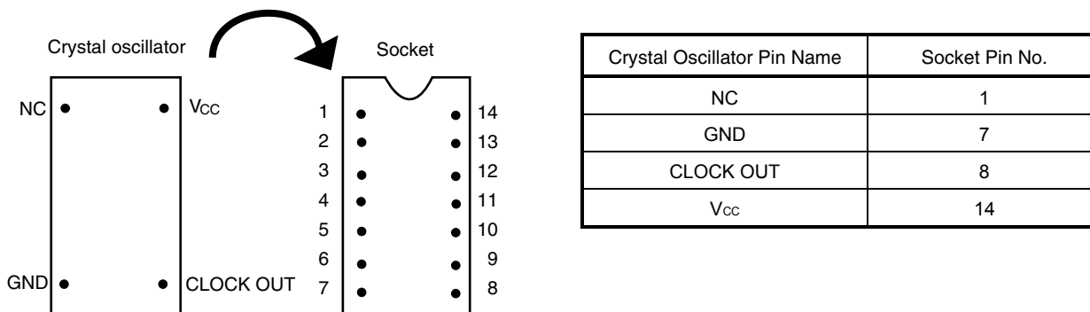
Figure 3-14. Pin Alignment of Crystal Oscillator and Socket
