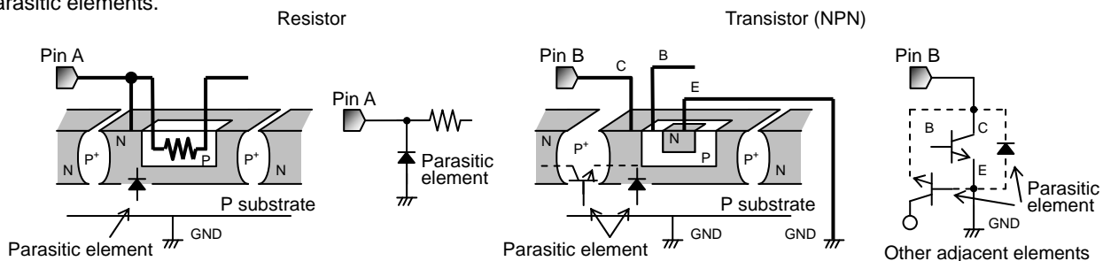
Fig.37 Simplified structure of monolithic IC
