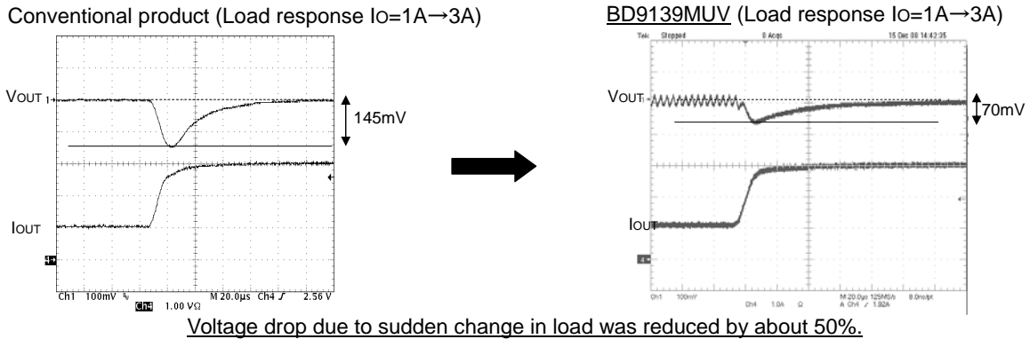
Fig.18 Comparison of transient response
