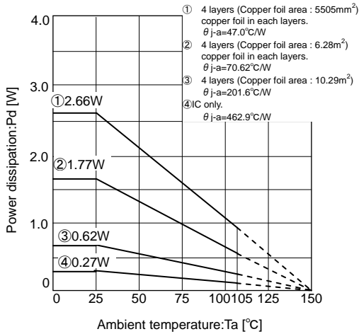
Fig.26 Thermal derating curve (VQFN016V3030)
