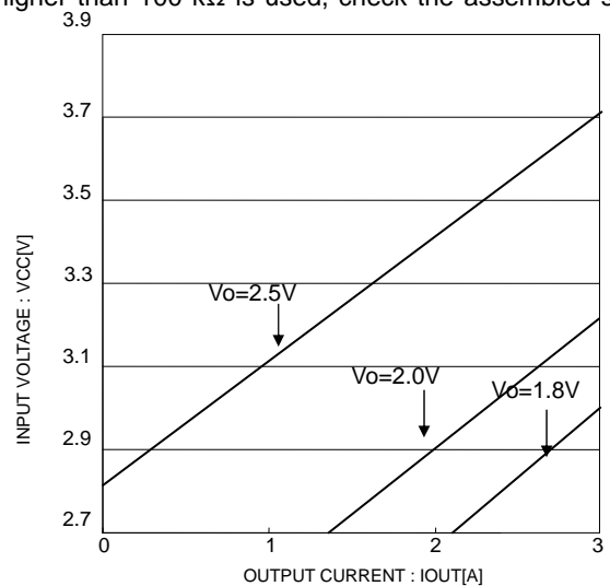
Fig.34 minimum input voltage in each output voltage
