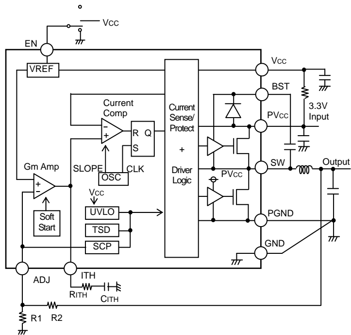
Fig.2 BD9139MUV Block Diagram
