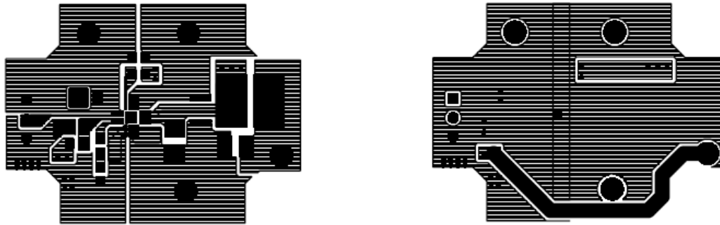
Fig.35 Layout diagram
