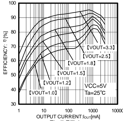
Fig.7 Efficiency
