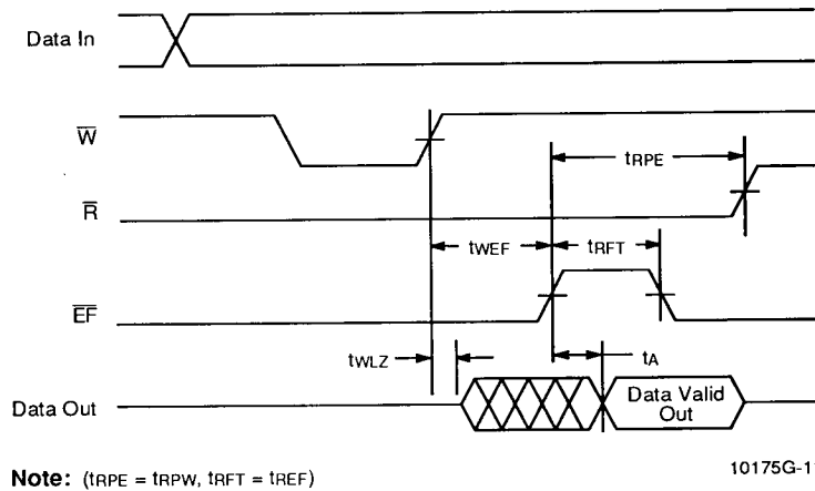
Figure 8. Read Data Flow-Through Mode
