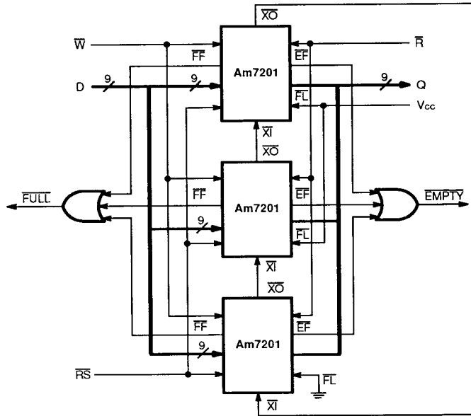
Figure 14. Depth-Expansion to Form 768 x 9 FIFO
