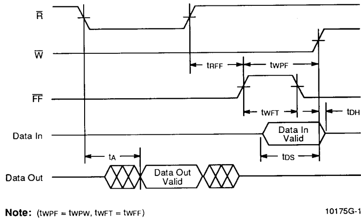
Figure 9. Write Data Flow-Through Mode
