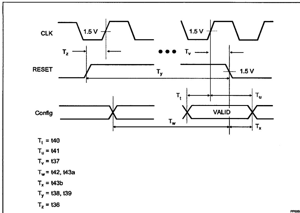
Figure 7. Reset and Configuration Timings
