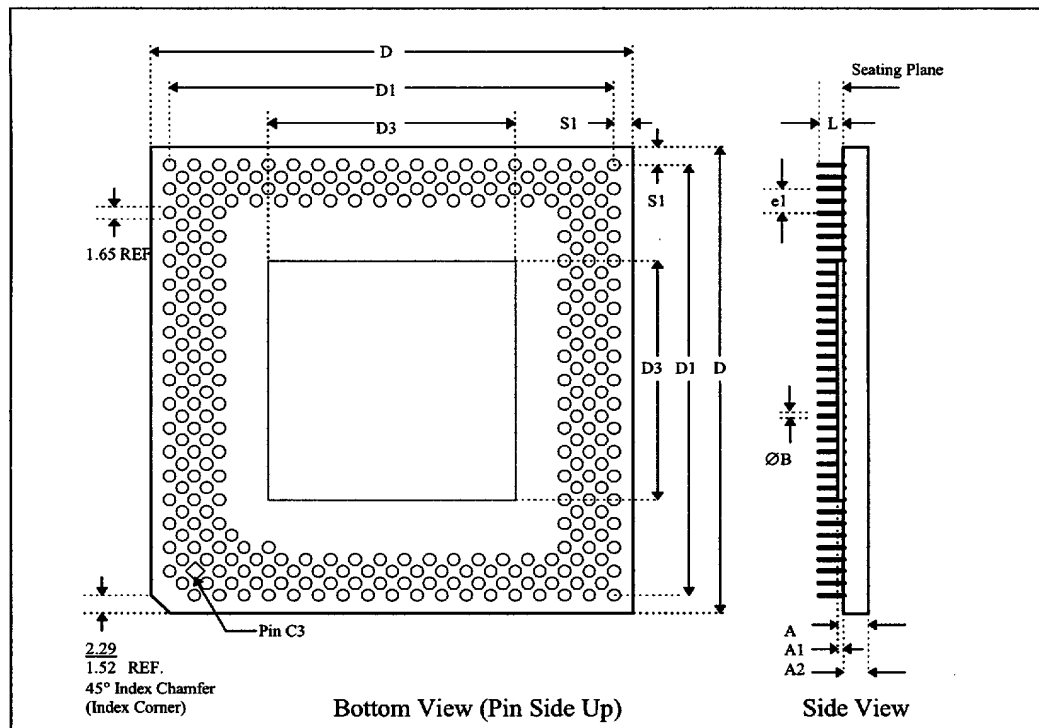
Figure 22. 296-Pin Ceramic Pin Grid Array Package
