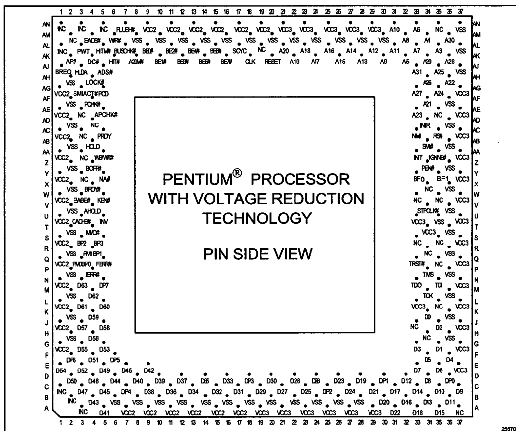
Figure 21. SPGA Pentium® Processor with Voltage Reduction Technology Pinout
