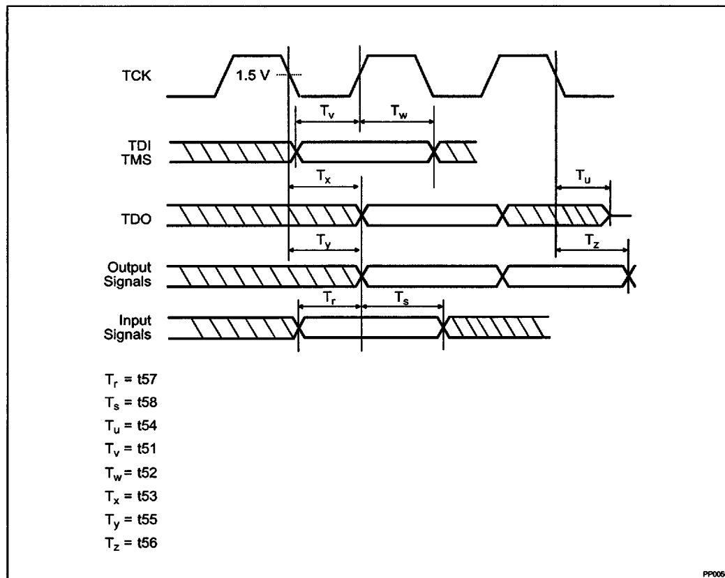
Figure 8. Test Timings
