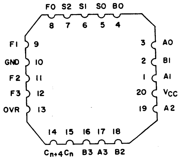
FIGURE 1. Terminal connections.
