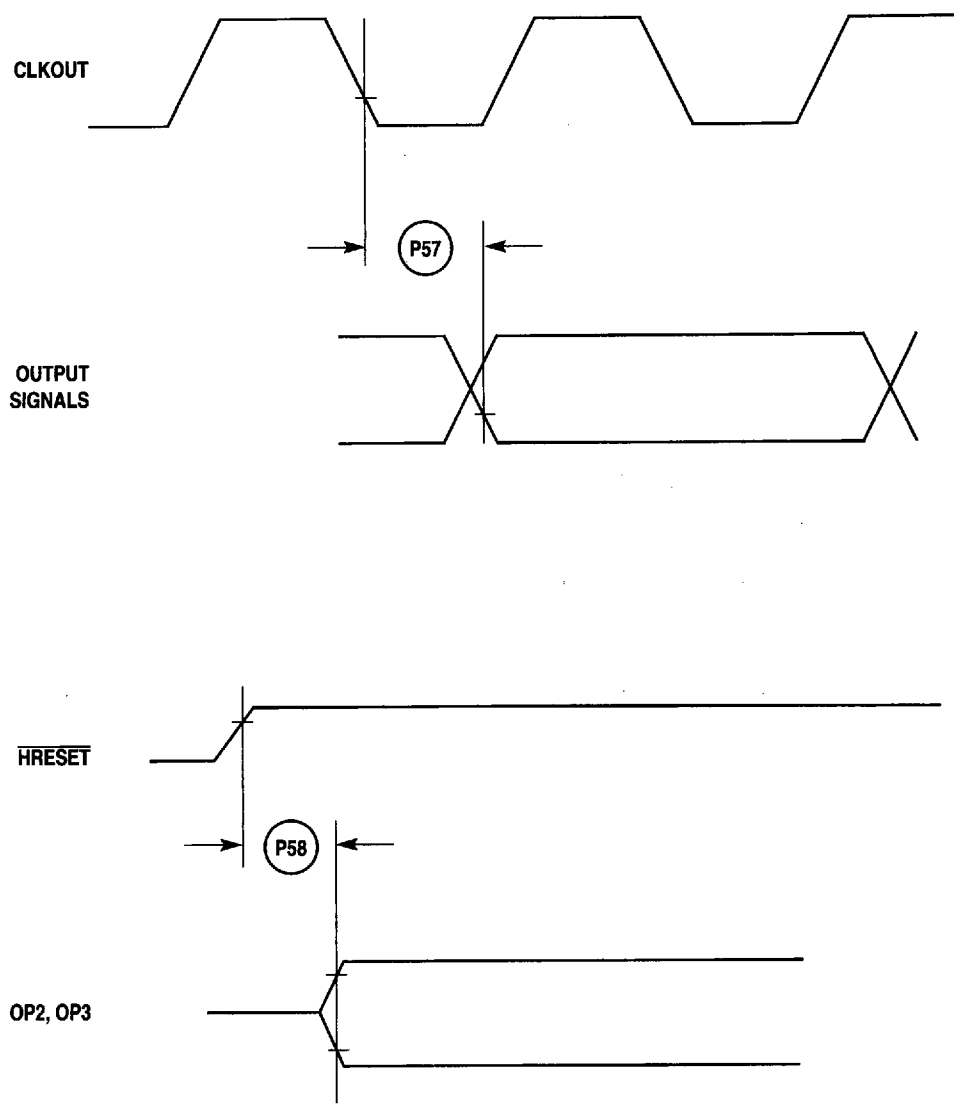
Figure 20-26. PCMCIA Output Port Timing Diagram
