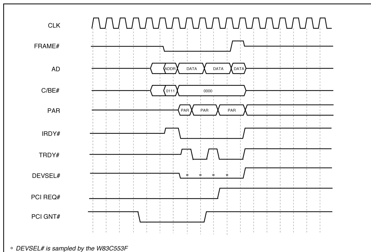
Figure 3-12. Preemption Timing
