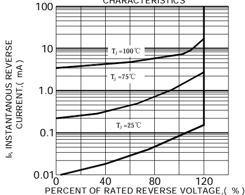
FIG.5-TYPICAL REVERSE CHARACTERISTICS
