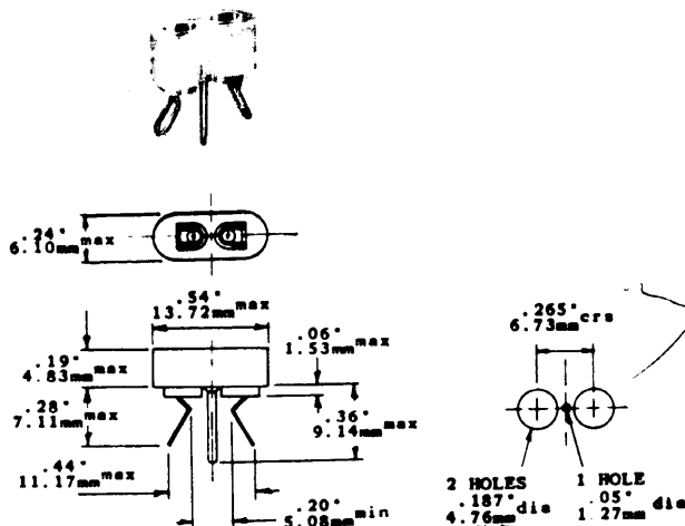
MOUNTING DETAILS
