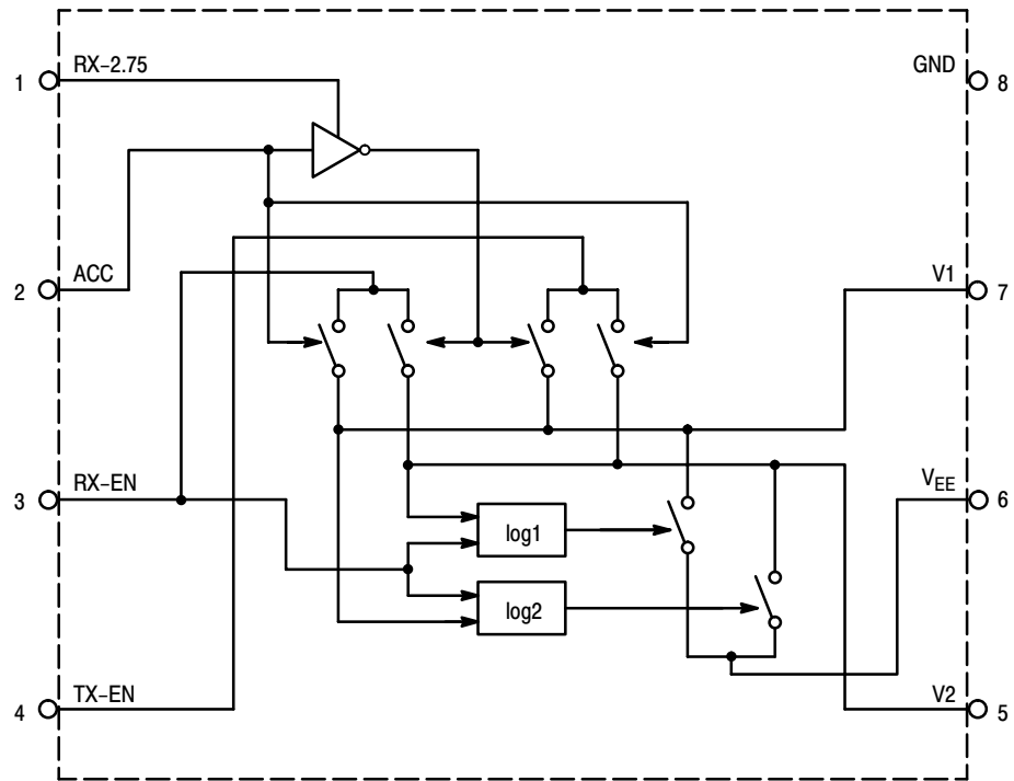
Figure 10. Antenna Switch Controller Block Diagram
