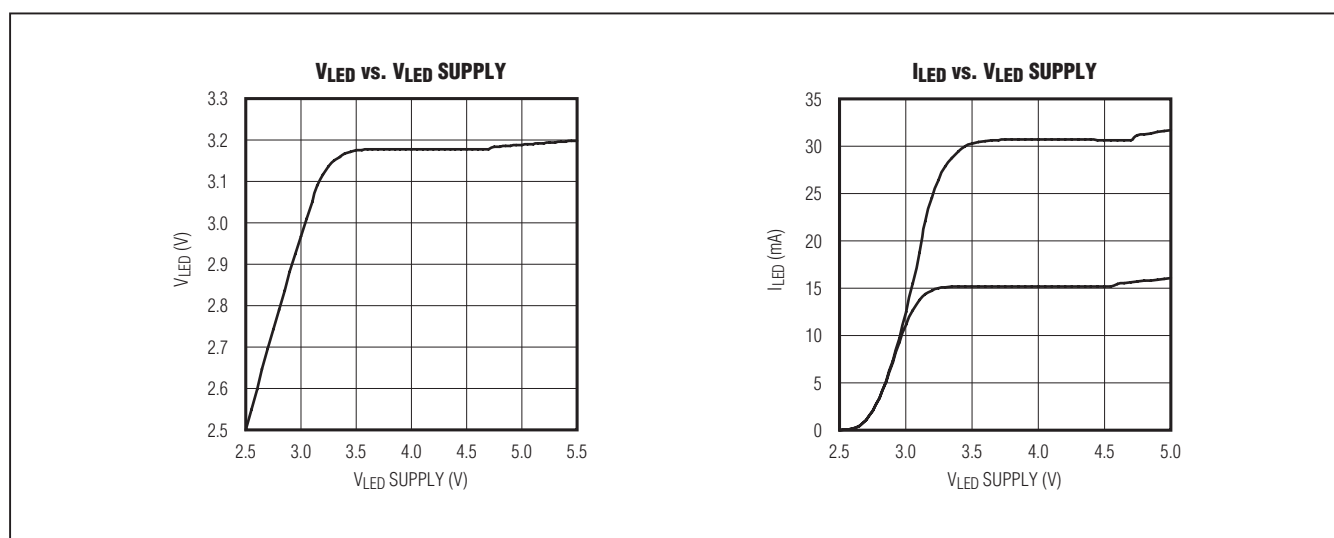
Figure 16. LED Brownout
