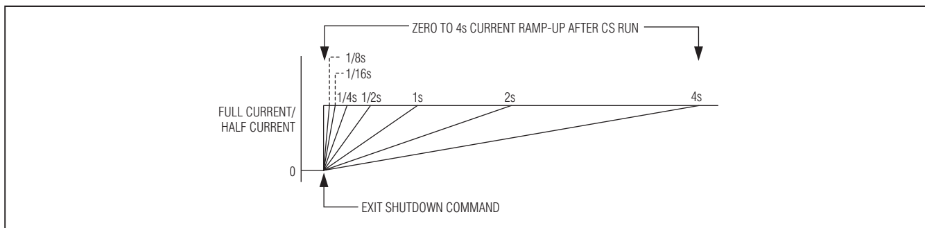
Figure 4. Ramp-Up Behavior
