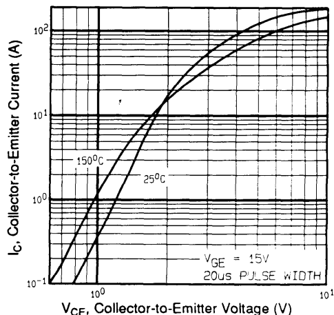
Fig. 2. Typical Output Characteristics T_J = 25^\circ\text{C} T_J = 150^\circ\text{C}
