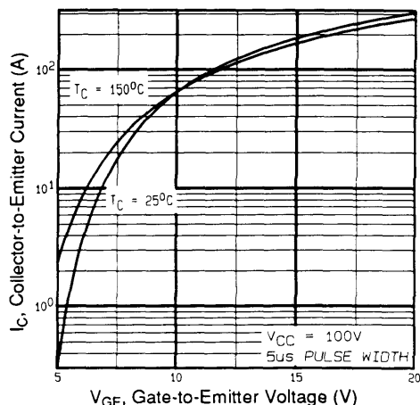
Fig. 3. Typical Transfer Characteristics T_J = 25^\circ\text{C} T_J = 150^\circ\text{C}
