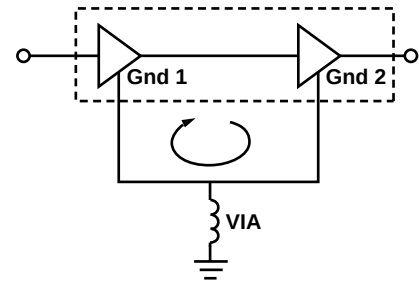
Figure 12. INA-32063 Potential Ground Loop.
