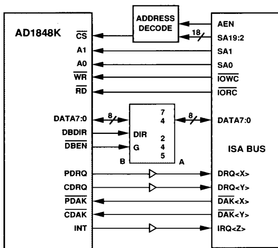
Figure 1. Interface to ISA Bus
