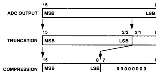
Figure 3. A-Law or \mu -Law Compression
