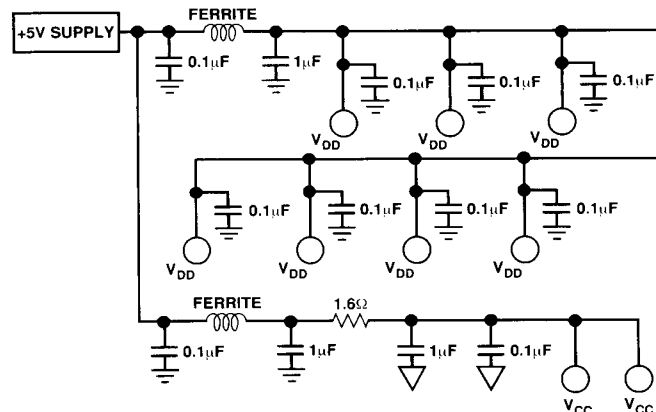
Figure 24. AD1848K Recommended Power Supply Bypassing
