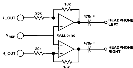
Figure 20. AD1848K Headphone Drive Connections
