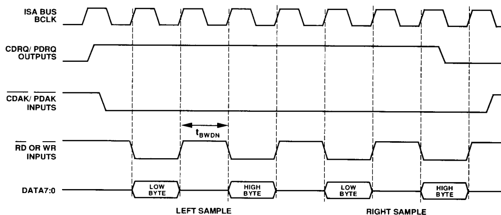
Figure 16. AD1848K 16-Bit Stereo DMA Cycle
