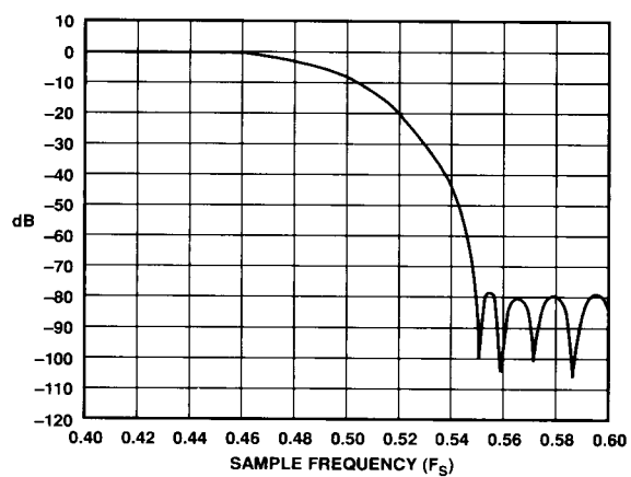
Figure 29. AD1848K Digital-to-Analog Frequency Response—Transition Band (Full-Scale Inputs, 0 dB Attenuation)
