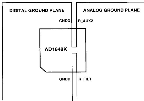
Figure 25. AD1848K Recommended Ground Plane
