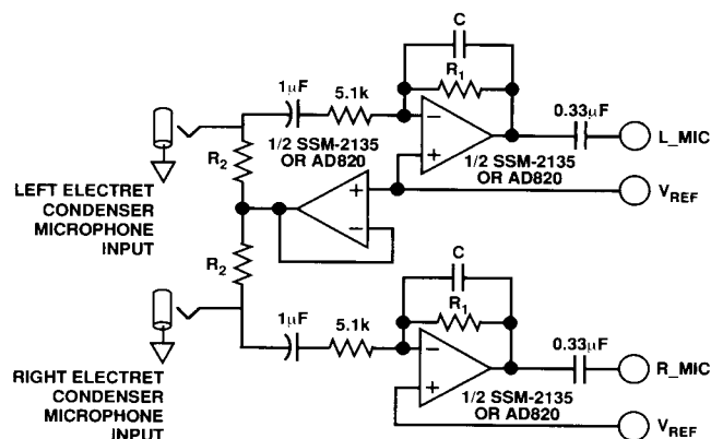
Figure 18. AD1848K "Phantom-Powered" Microphone Input Circuit
