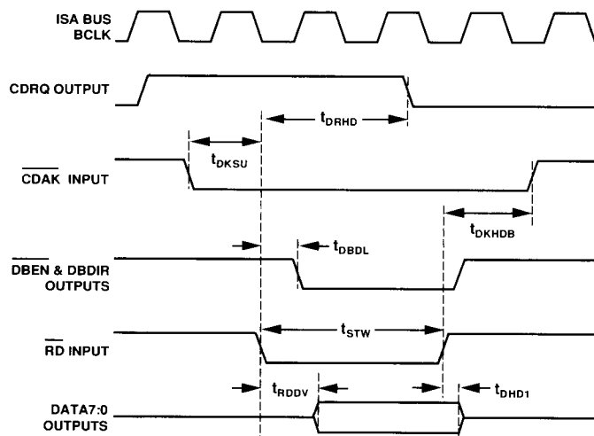
Figure 13. AD1848K 8-Bit Mono DMA Read/Capture Cycle
