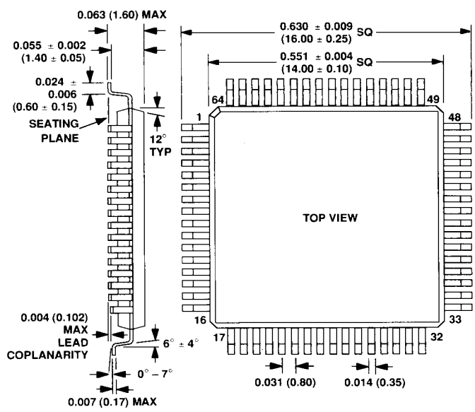
ST-64 64-Lead Thin Quad Flatpack
