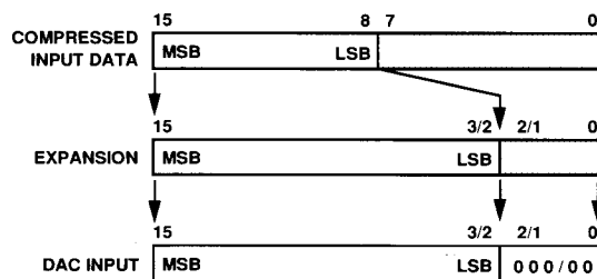
Figure 2. A-Law or \mu -Law Expansion
