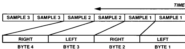
Figure 8. AD1848K 8-Bit Stereo Data Stream Sequencing
