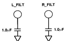
Figure 22. AD1848K External Filter Capacitor Connections
