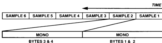
Figure 9. AD1848K 16-Bit Mono Data Stream Sequencing
