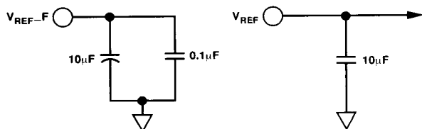
Figure 21. AD1848K Voltage Reference Bypassing
