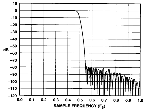
Figure 28. AD1848K Digital-to-Analog Frequency Response (Full-Scale Inputs, 0 dB Attenuation)
