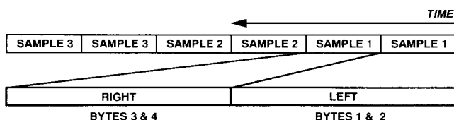
Figure 10. AD1848K 16-Bit Stereo Data Stream Sequencing
