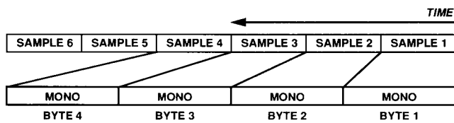
Figure 7. AD1848K 8-Bit Mono Data Stream Sequencing
