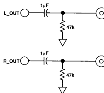
Figure 19. AD1848K Line Output Connections
