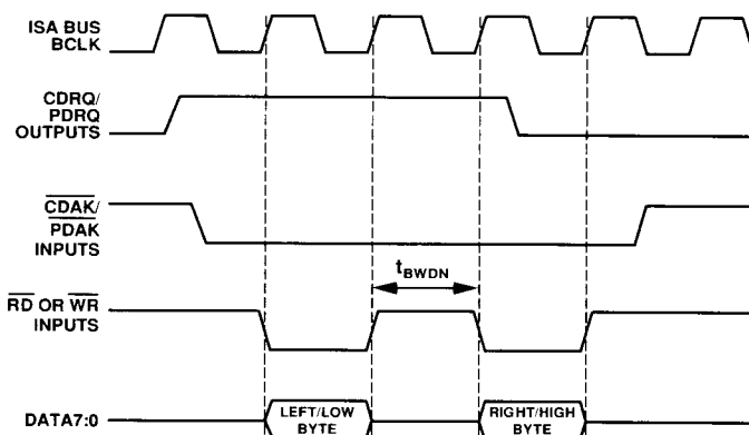
Figure 15. AD1848K 8-Bit Stereo or 16-Bit Mono DMA Cycle
