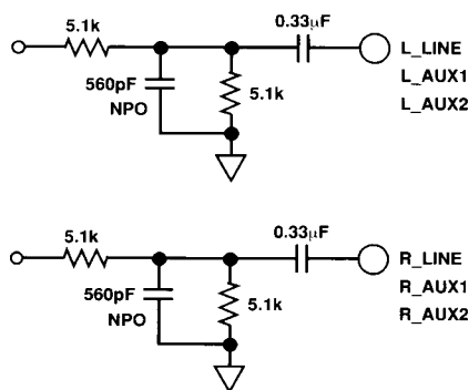
Figure 17. AD1848K 2 V rms Line-Level Input Circuit
