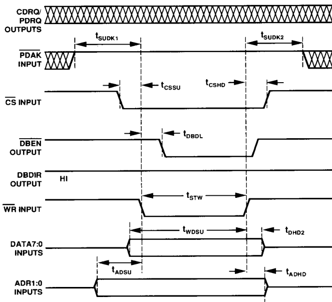
Figure 12. AD1848K Control Register/PPIO Write Cycle
