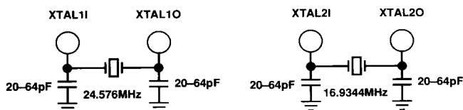
Figure 23. AD1848K Crystal Connections
