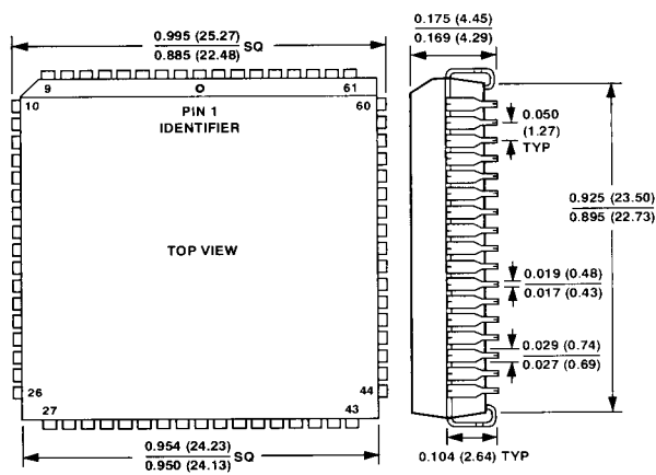
P-68 68-Lead Plastic Leaded Chip Carrier
