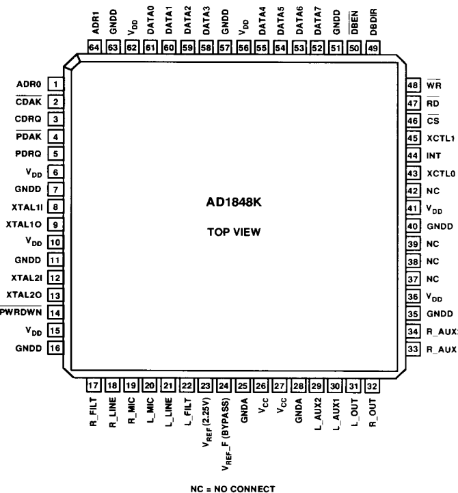
64-Lead Thin Quad Flatpack Pinout
