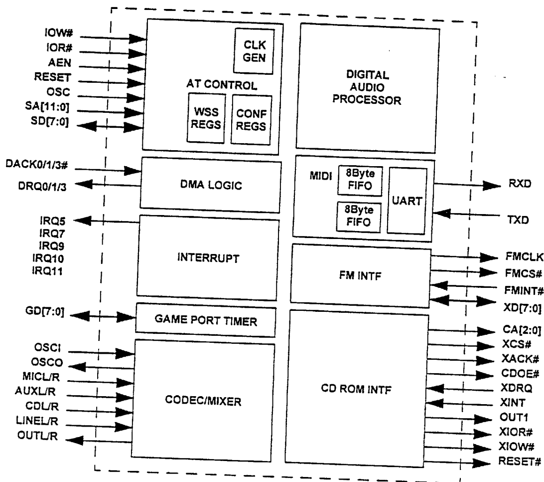
Figure 1-1 Block Diagram
