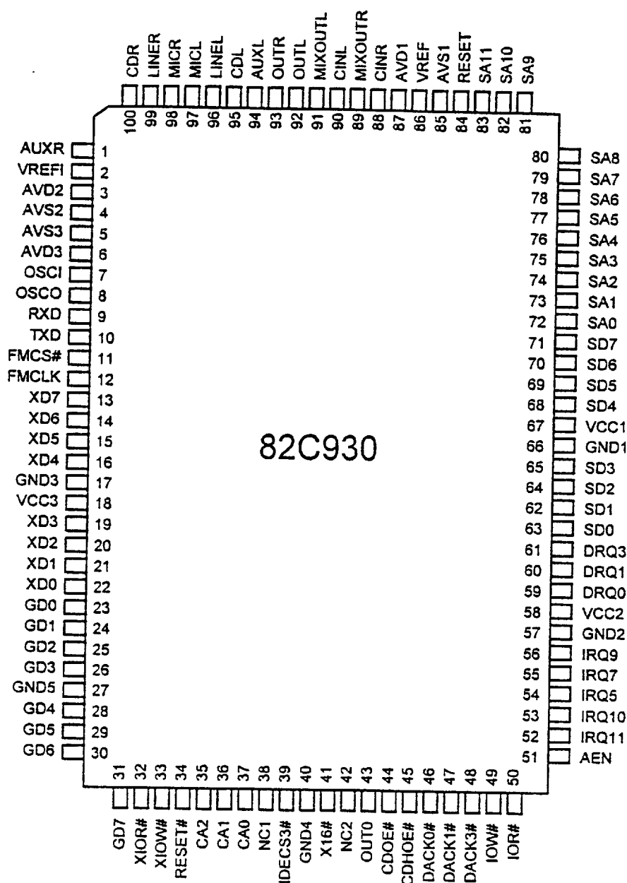
Figure 3-1 Pin Diagram
