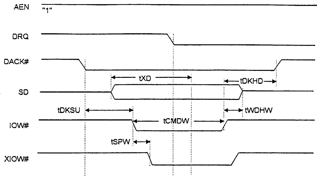
Figure 8-2 DMA Write/Playback Cycle
