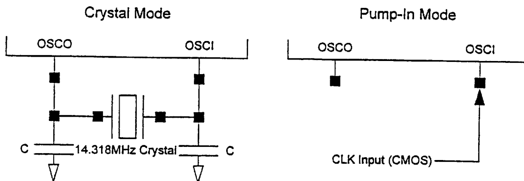
Figure 3-2 External Components
