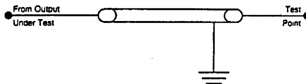
Figure 5. Transient Equivalent Testing Load Circuit ( V_{CC} = 3.3V )
