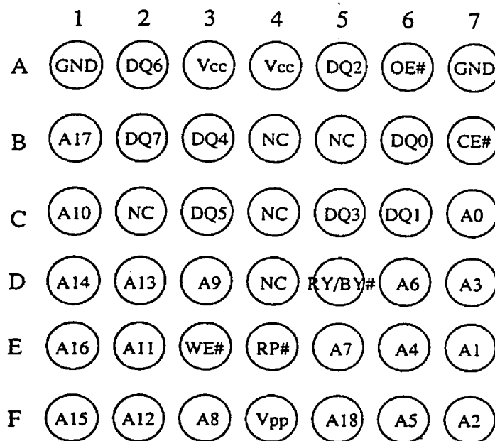
LH28F004SUB - Z9 (Top View)
