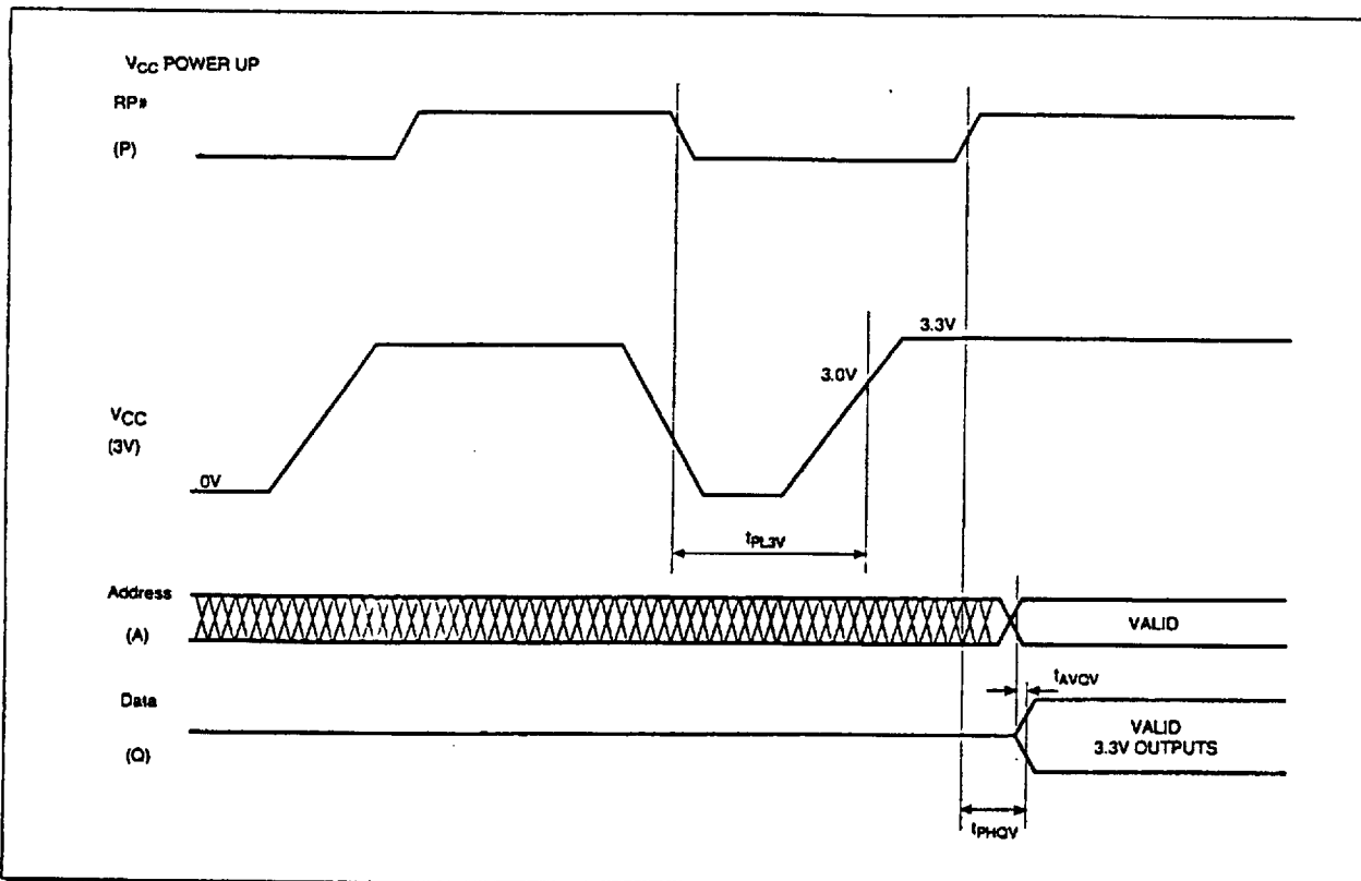
Figure 7. V_{CC} Power-Up and RP\# Reset Waveforms
