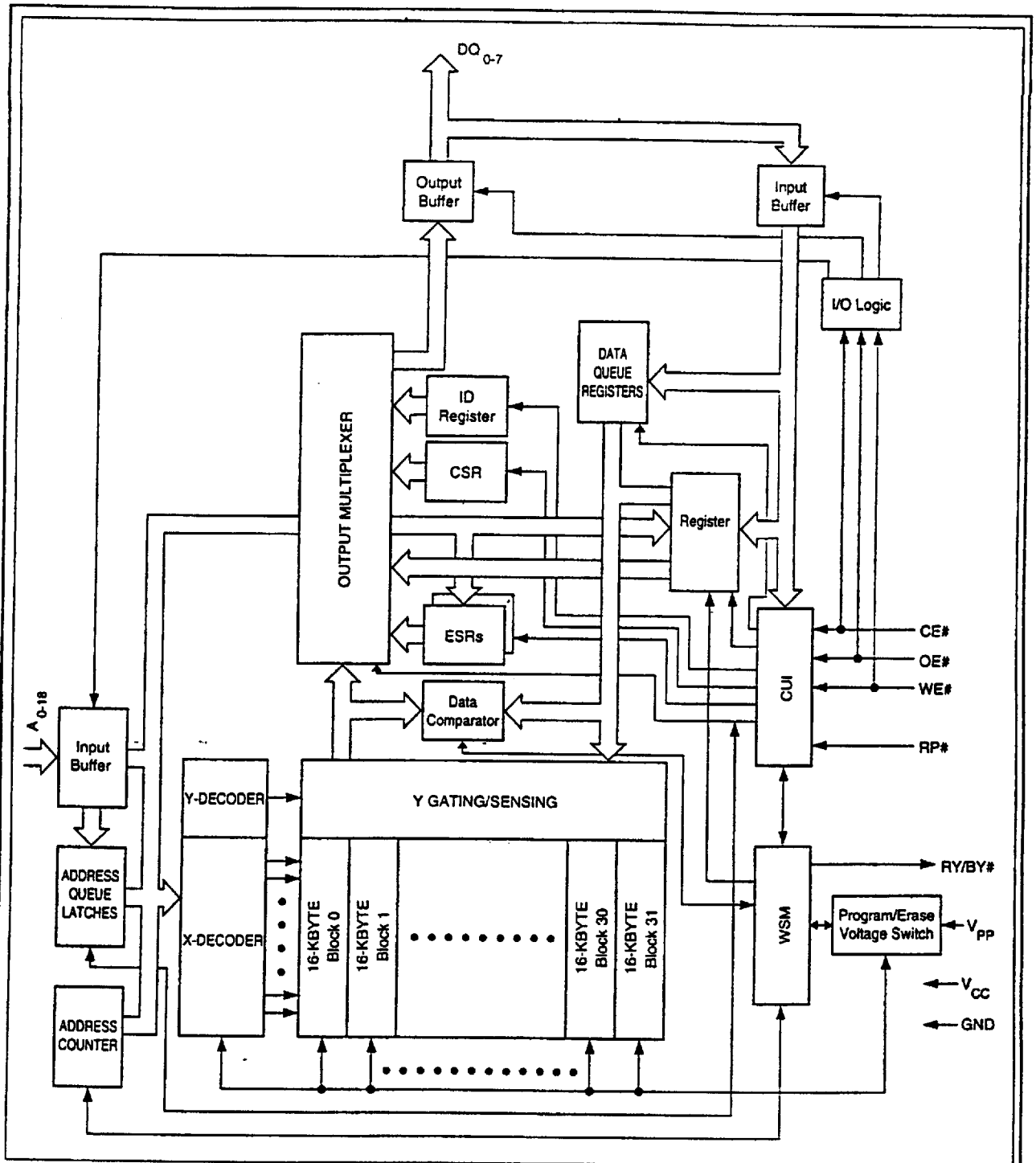
Figure 1. LH28F004SUB-Z9 Block Diagram
