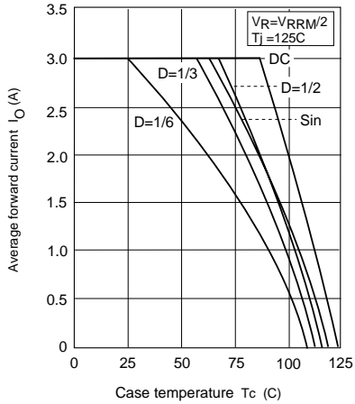
Fig.6 Average forward current Vs. Case temperature
