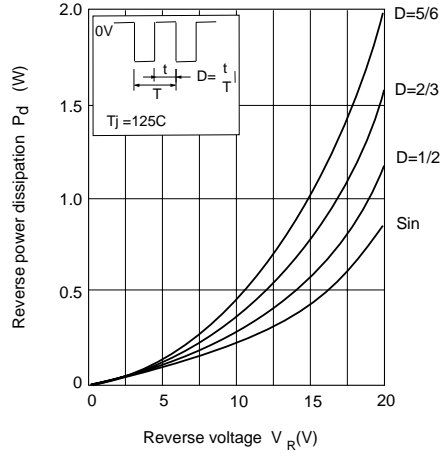
Fig.5 Reverse power dissipation Vs. Reverse voltage
