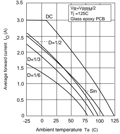
Fig.7 Average forward current Vs. Ambient temperature
