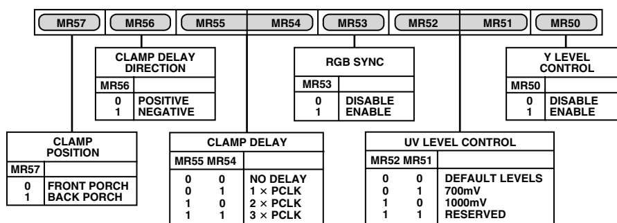
Figure 61. Mode Register 5, MR5
