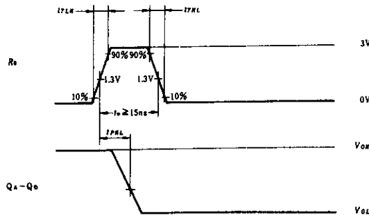
Waveform-2 t_{PHL} (R 0 →Q)
