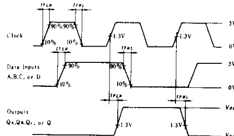
Waveform-2 t_{PLH} , t_{PHL} (Clock → Q)
