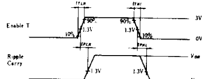
Waveform-3 t_{PLH} , t_{PHL} (Enable T → Ripple Carry)
