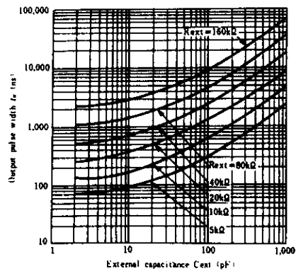
Fig.3 Typical Output Pulse Width ( C_{ext} \leq 1000\text{pF} )
