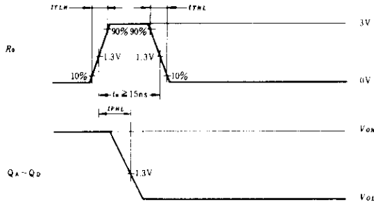
Waveform-2 t_{PHL} (R 0 \rightarrow Q)
