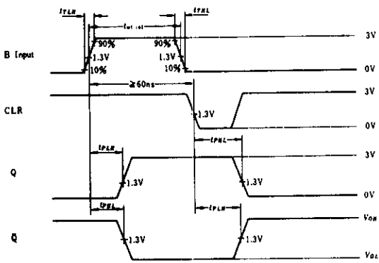
Trigger from B, then clear (A input is low).
