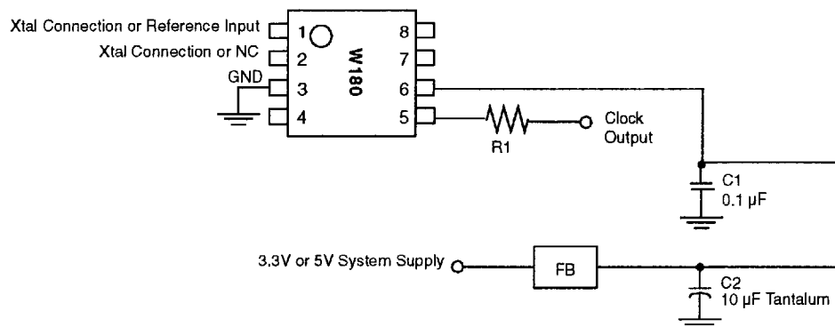
Figure 4. Recommended Circuit Configuration
