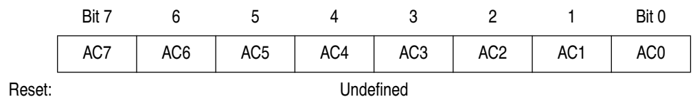
Figure 8. MCAN Acceptance Code (CACC)
