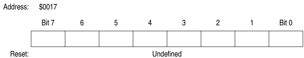
Figure 11. Output Compare Low Register (OCL)
