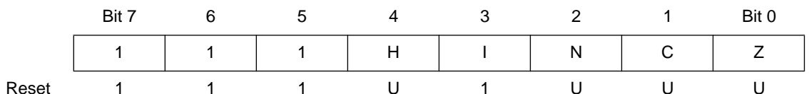
Figure 6. Condition Code Register
