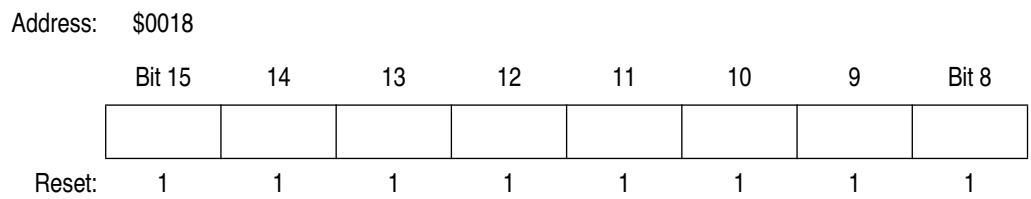
Figure 2. Timer Counter High Register (TCH)
