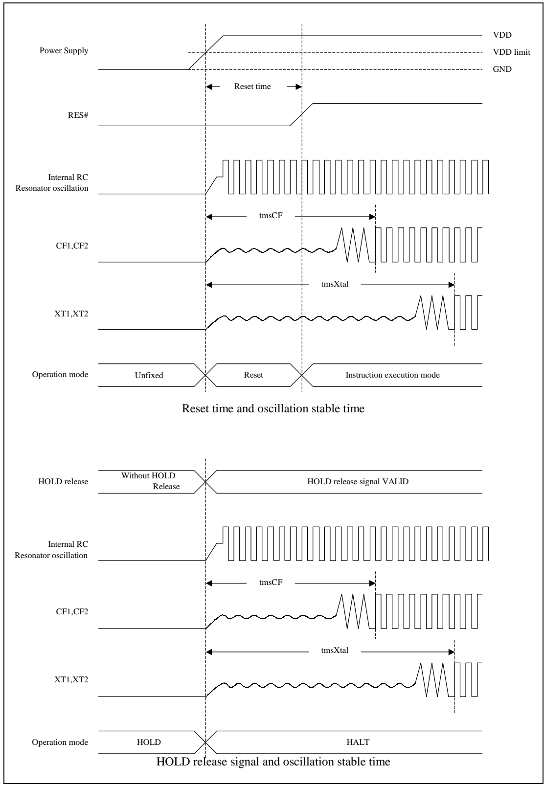
Figure 4 Oscillation stabilizing time
