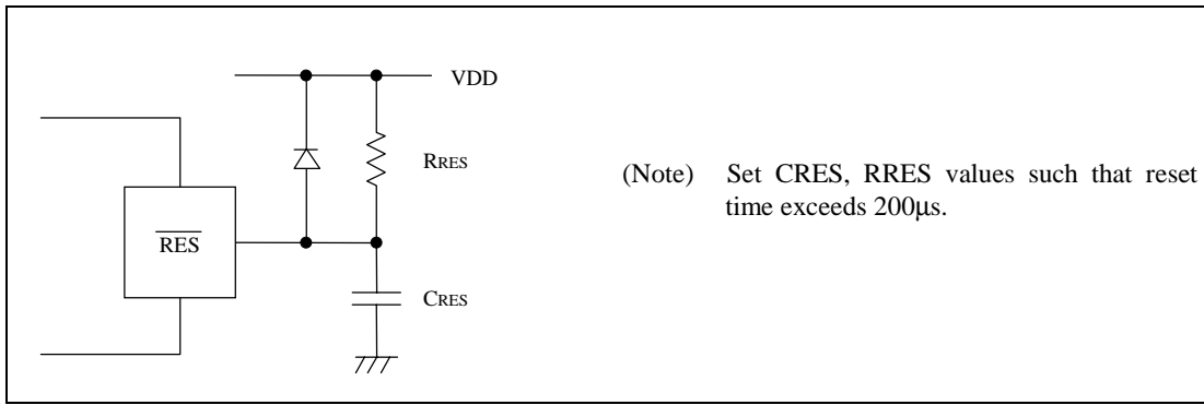
Figure 5 Reset circuit
