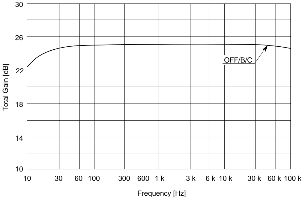
Total Gain vs. Frequency (REC MODE PBOUT V_{cc} = 14 V )
