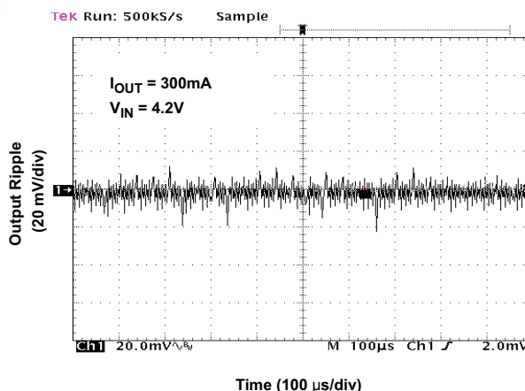
Figure 20. Output Ripple
