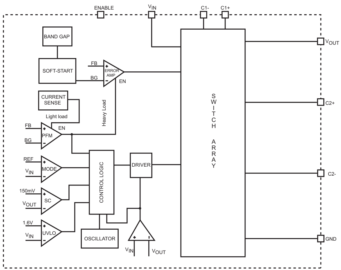
Figure 2. Block Diagram
