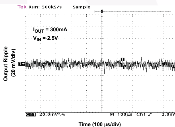
Figure 18. Output Ripple
