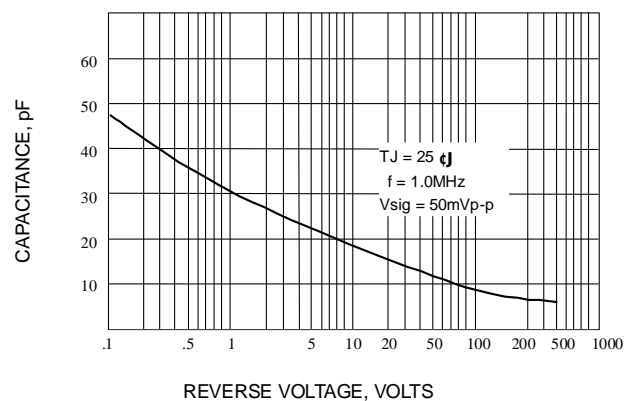
Fig. 6-TYPICAL JUNCTION CAPACITANCE
