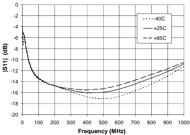
|S11| (dB) vs. Frequency
