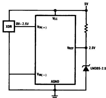
FIGURE 3b. Absolute with a Reduced Span
