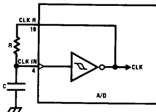
FIGURE 2. Self-Clocking the A/D
