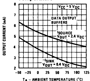
Output Current vs Temperature
