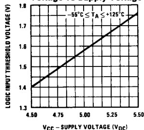
Logic Input Threshold Voltage vs Supply Voltage
