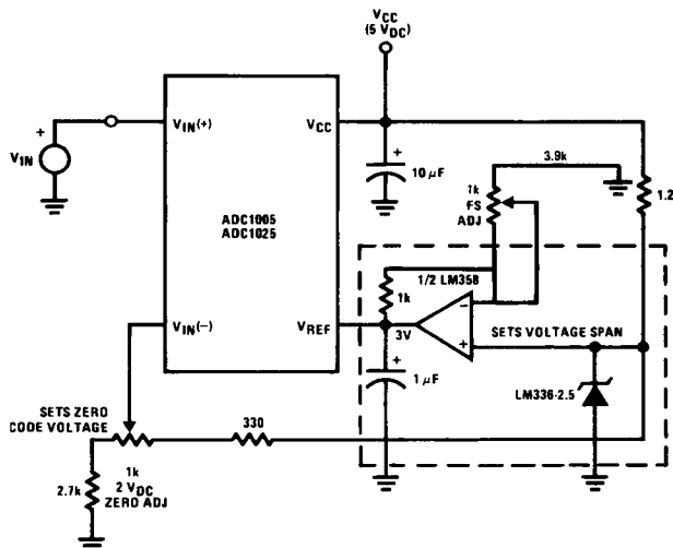
Figure 4. Zero-Shift and Span-Adjust ( 2\text{V} \leq V_{IN} \leq 5\text{V} )
