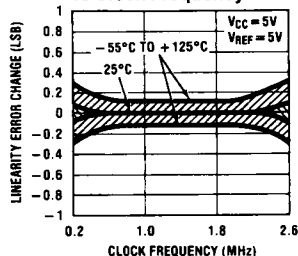
Typical Linearity Error vs Clock Frequency
