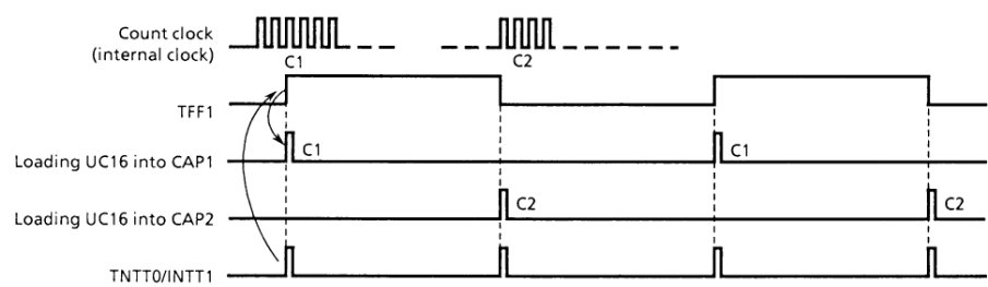
Figure 3.8 (12). Frequency Measurement
