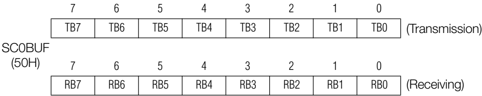
Figure 3.10 (5). Serial Transmission/Receiving Buffer Registers (Channel 0, SC0BUF)
