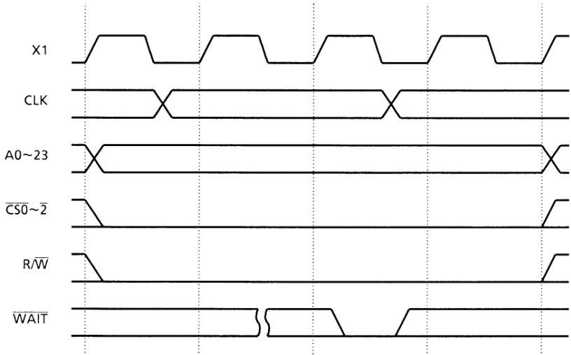
Figure 3.13 (1). DRAM Controller
