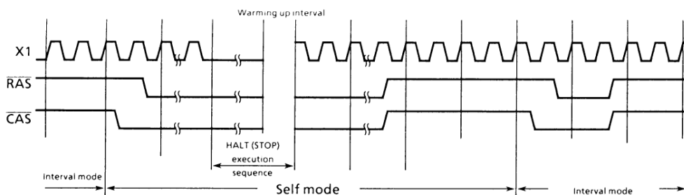
Figure 3.13 (8). Self Refresh Cycle Timing
