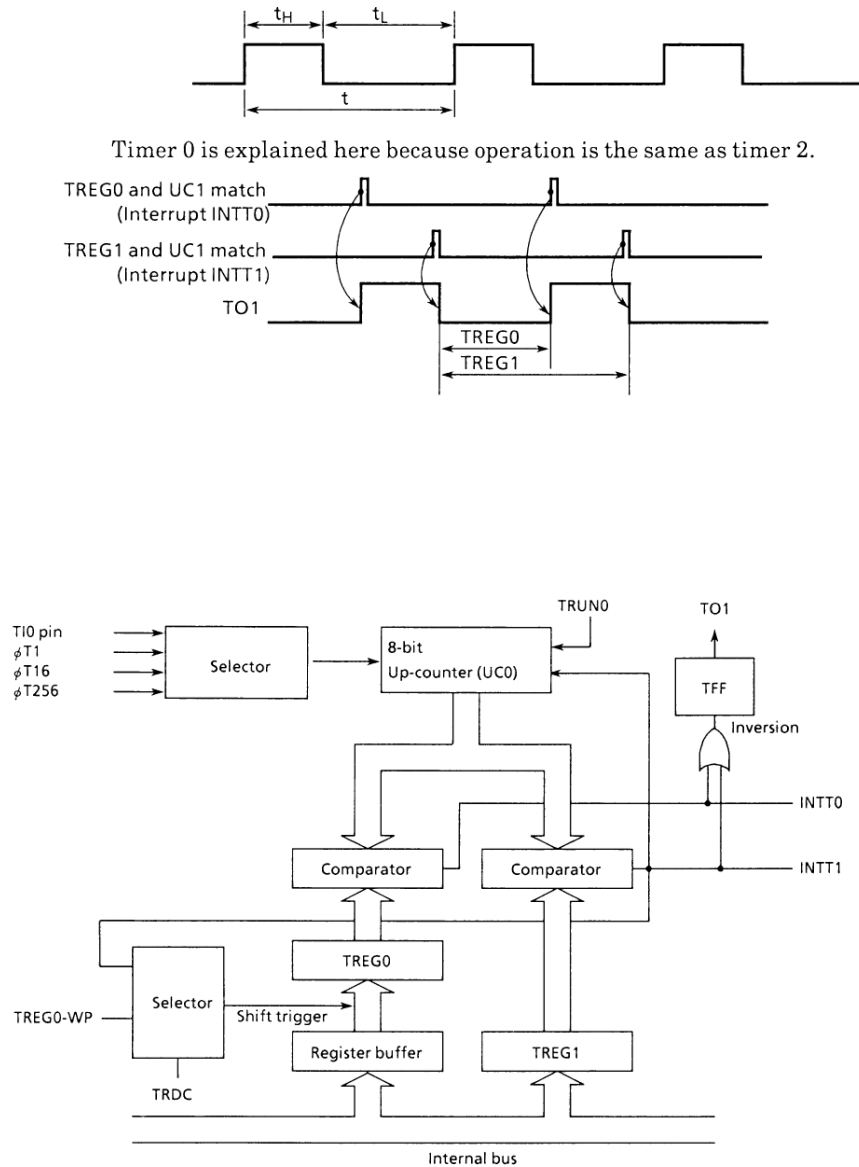
Figure 3.7 (12). Block Diagram of 8-Bit PPG Output Mode
