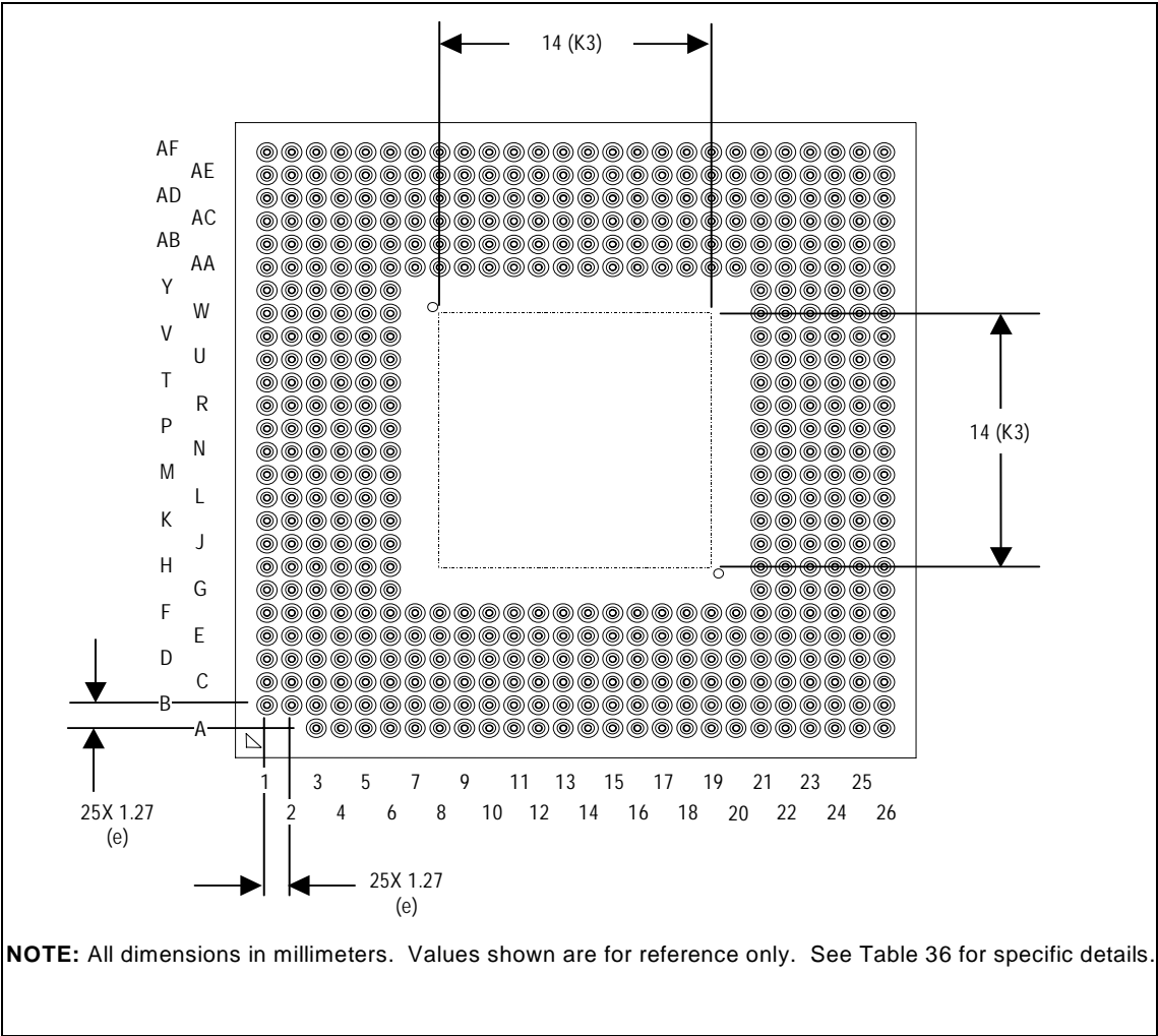
Figure 24. Socketable Micro-FCPGA Package - Bottom View
