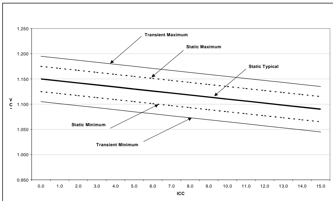
Figure 4. Illustration of V_{CC} Static and Transient Tolerances (VID = 1.15 V)
