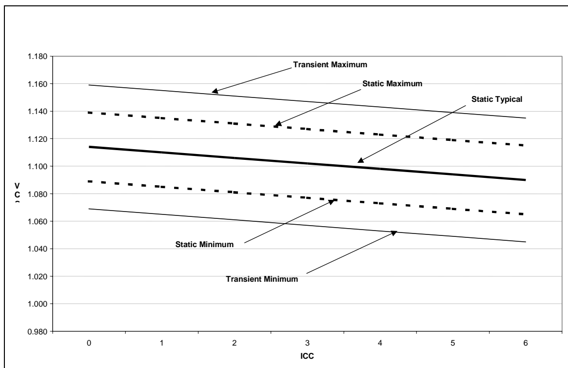
Figure 5. Illustration of Deep Sleep V_{CC} Static and Transient Tolerances (VID Setting = 1.15 V)
