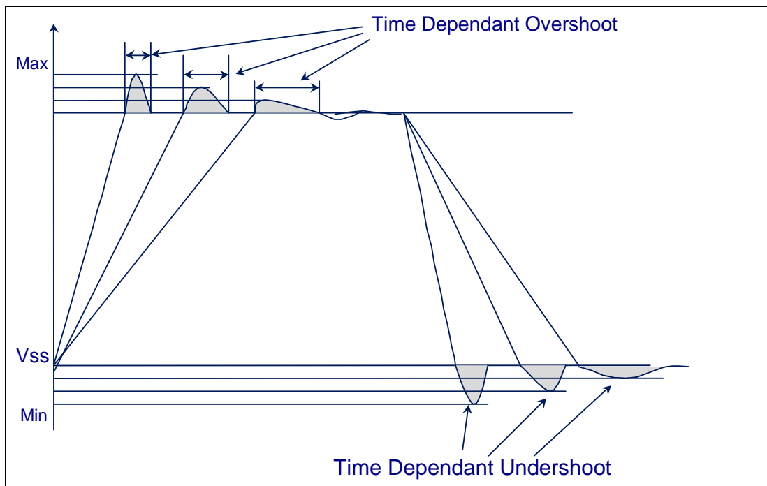
Figure 20. Maximum Acceptable Overshoot/Undershoot Waveform
