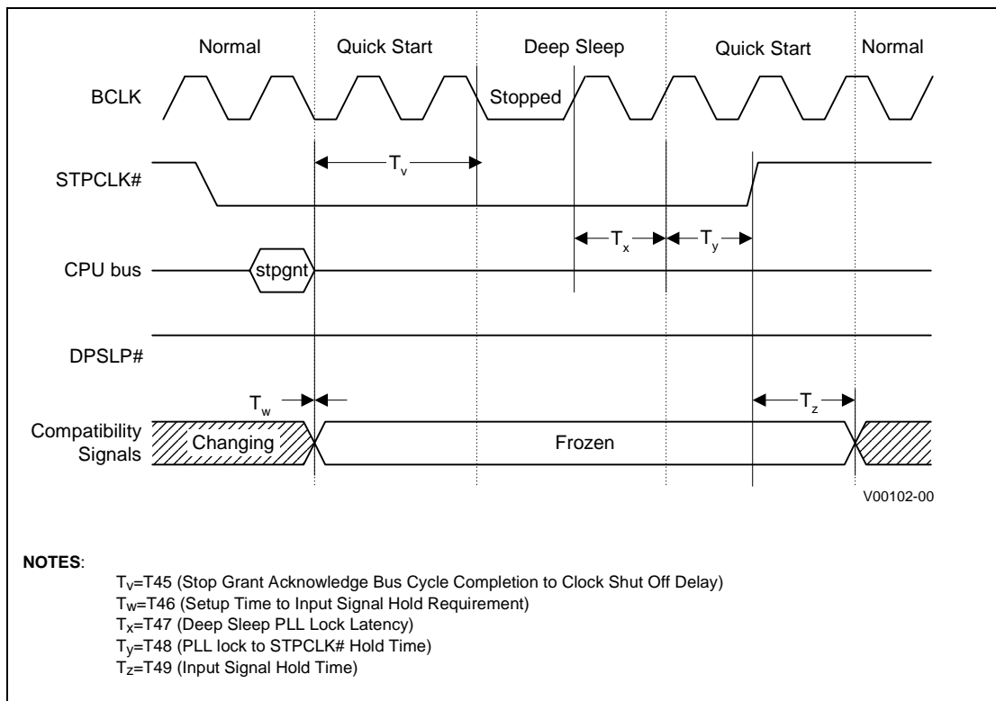
Figure 17. Quick Start/Deep Sleep Timing (BCLK Stopping Method)
