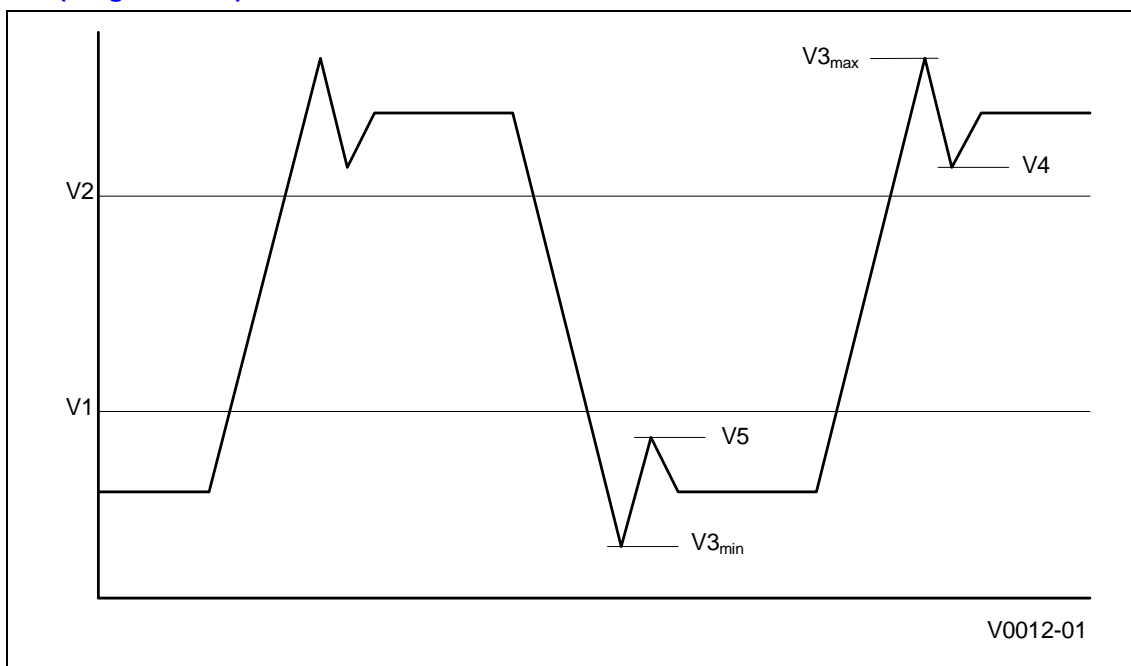
Figure 19. BCLK (Single Ended)/PICCLK Generic Clock Waveform
