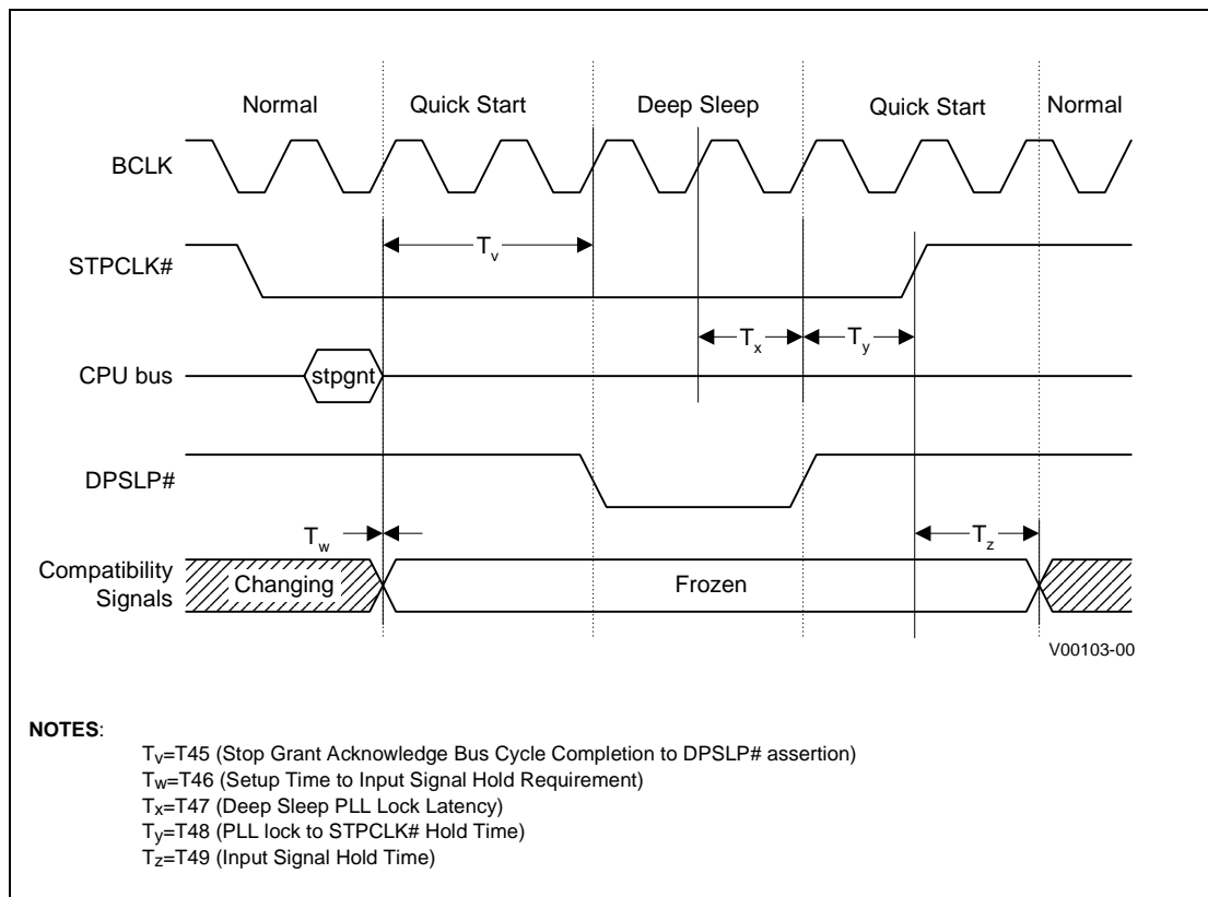
Figure 18. Quick Start/Deep Sleep Timing (DPSLP# Assertion Method)
