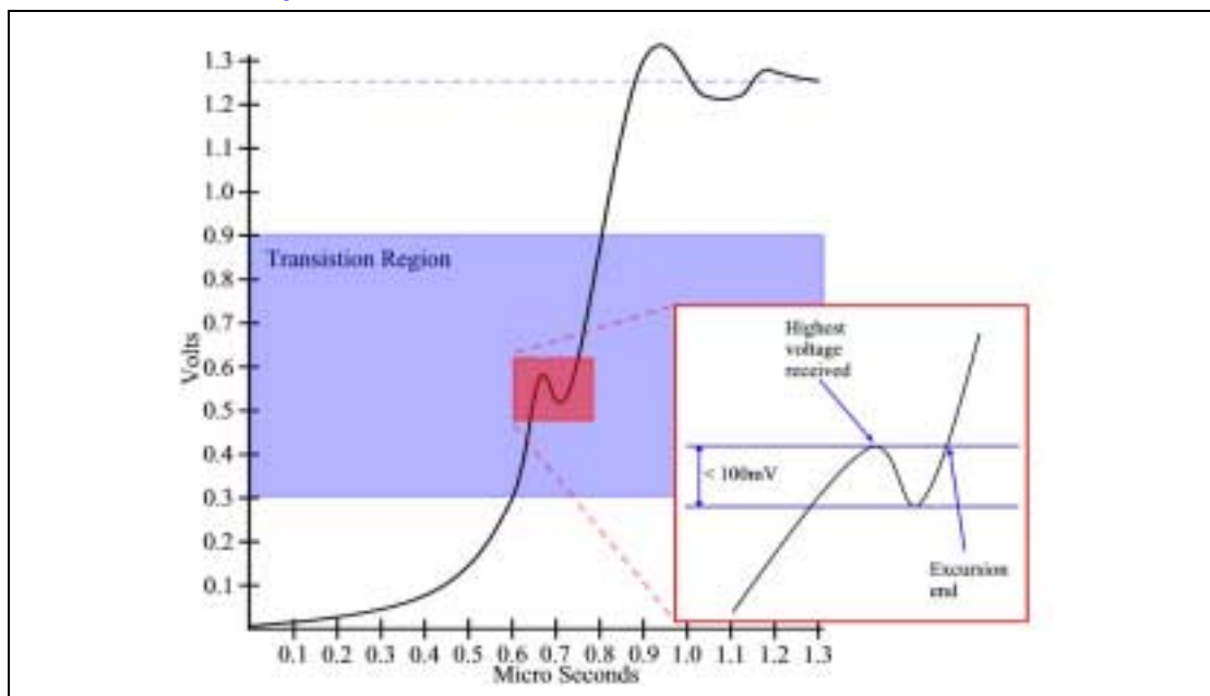
Figure 21. VTT_PWRGD Noise Specification
