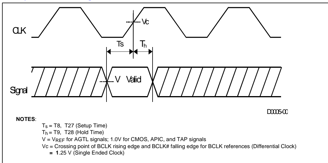
Figure 10. Setup and Hold Timings
