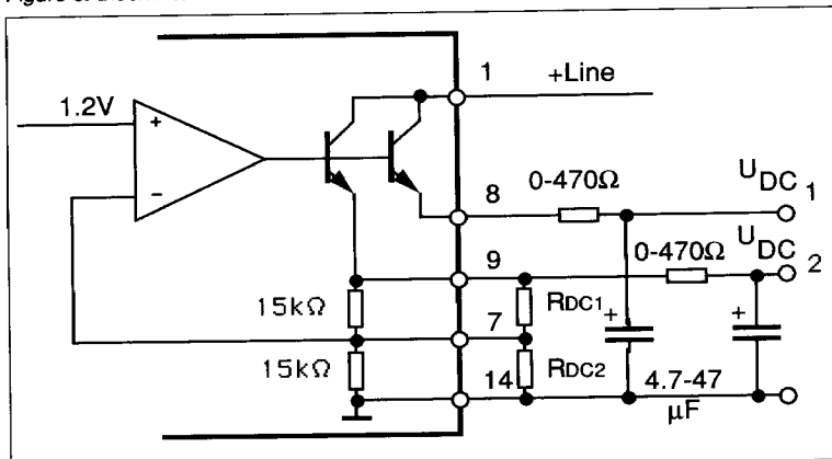
Figure 7. DC regulator for external CMOS devices.
