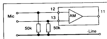
Figure 15. Additional components for extended low current/voltage operation.
