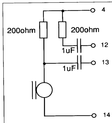
Figure 14. Electret microphone with FET-buffer, e.g. EM80.
