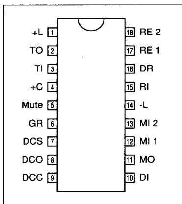
Figure 5. Pin configuration.
