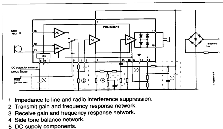
Figure 1. Functional diagram.
