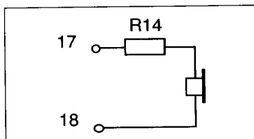
Figure 13. Magnetic receiver connection.
