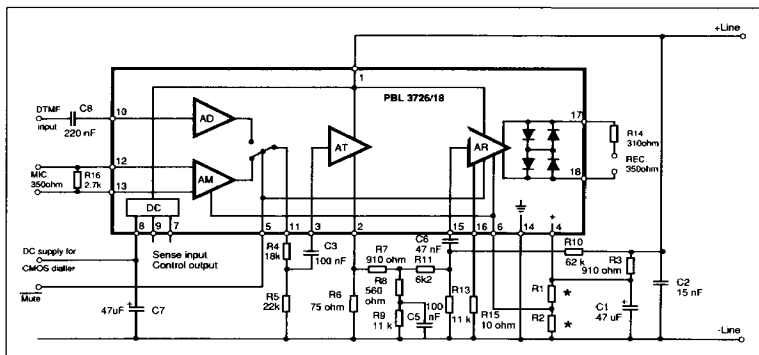
Figure 4. Circuit with external components for test setup.
