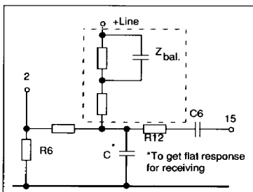
Figure 12. Sidetone network especially suited for applications with a high line current, when R6 has a low value.
