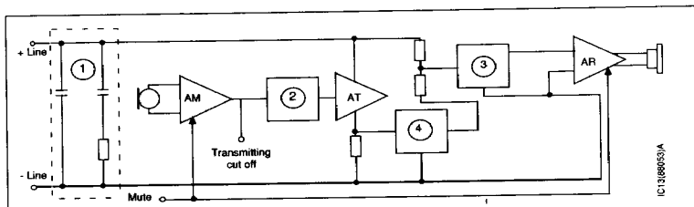
Figure 6. Block interconnections.
