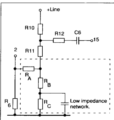
Figure 11. Typical sidetone network.
