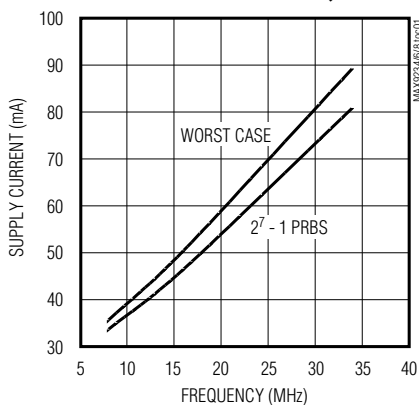
MAX9234/MAX9236 WORST-CASE PATTERN AND PRBS SUPPLY CURRENT vs. FREQUENCY
