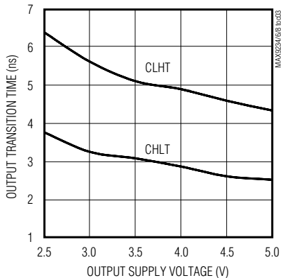
MAX9234/MAX9236 RxOUT TRANSITION TIME vs. OUTPUT SUPPLY VOLTAGE ( V_{CCO} )
