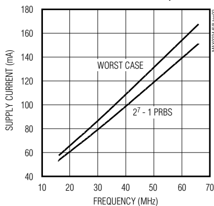
MAX9238 WORST-CASE PATTERN AND PRBS SUPPLY CURRENT vs. FREQUENCY
