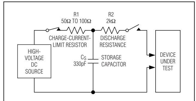
Figure 13. ISO 10605 Contact Discharge ESD Test Circuit
