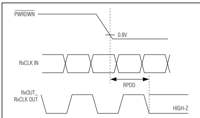
Figure 8. Power-Down Delay
