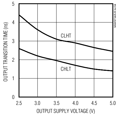
MAX9238 RxOUT TRANSITION TIME vs. OUTPUT SUPPLY VOLTAGE ( V_{CCO} )
