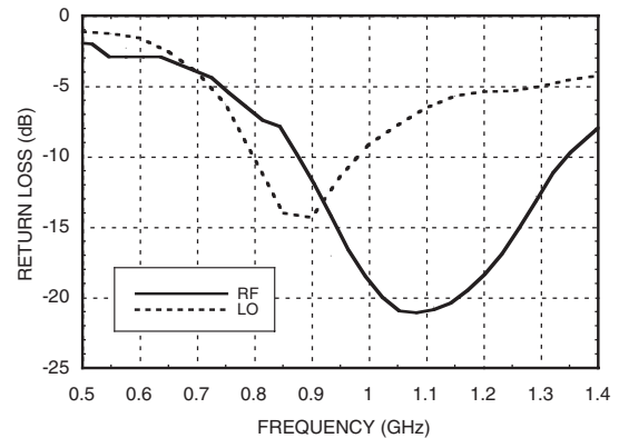
Return Loss @ LO = +19 dBm
