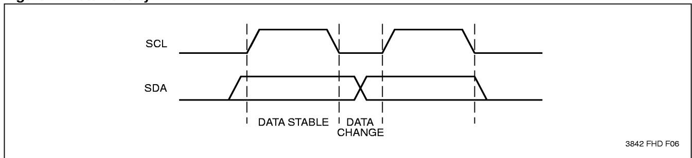
Figure 1. Data Validity
