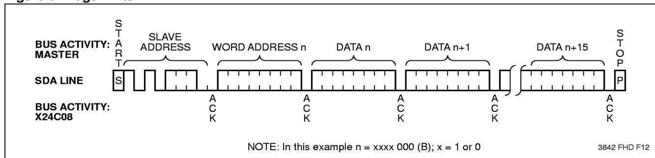
Figure 6. Page Write
