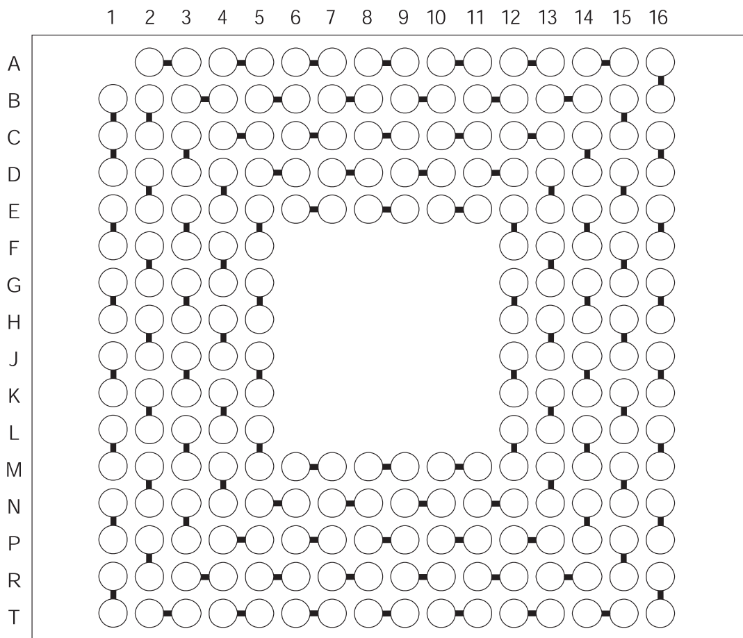
FIG. 1: DAISY-CHAIN INTERCONNECTION
