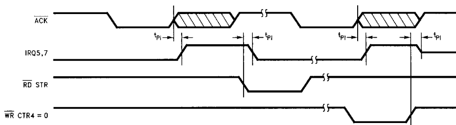
FIGURE 11-19. Extended Mode Parallel Port Interrupt Timing
