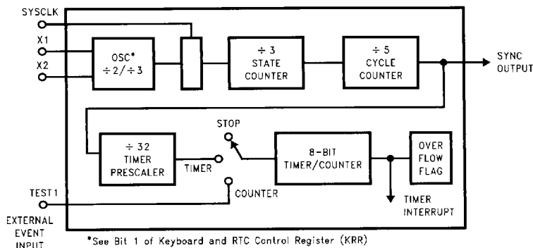
FIGURE 9-10. Timing Generation and Timer Circuit
