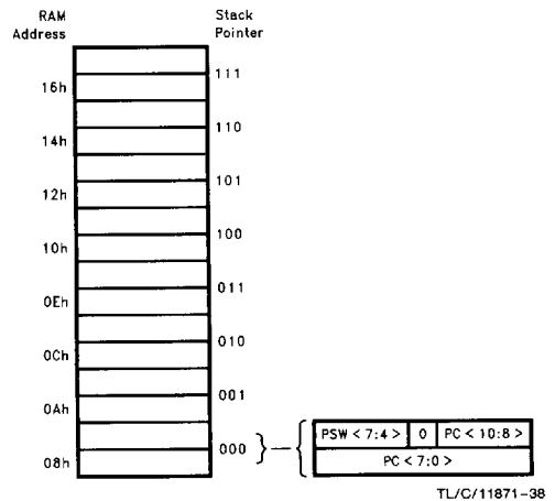
FIGURE 9-6. Keyboard Controller Stack Organization
