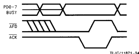
FIGURE 7-7. ECP Backward Read Cycle
