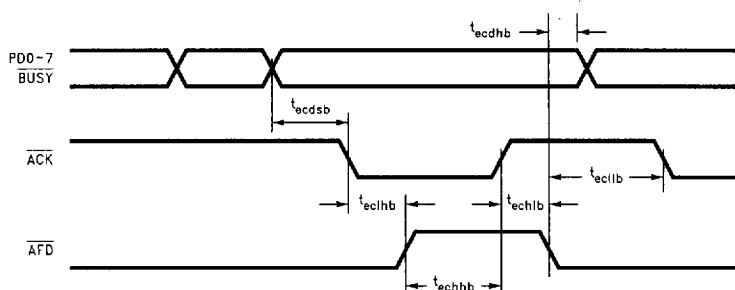
FIGURE 11-23. ECP Parallel Port Backward Timing Diagram
