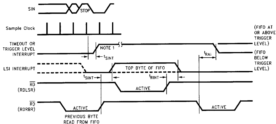
FIGURE 11-10. Timeout Receiver Timing
