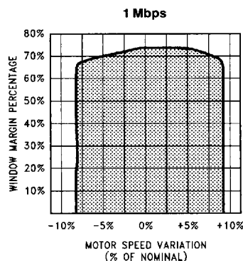
FIGURE 5-2. PC87323 Dynamic Window Margin Performance
