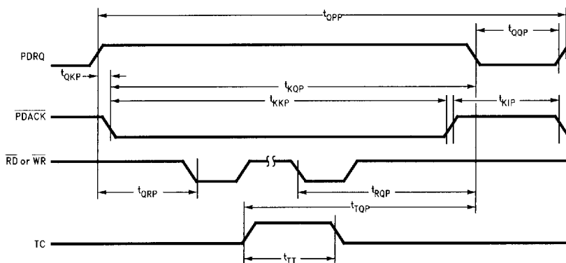
FIGURE 11-12b. ECP DMA Timing
