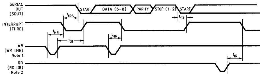
FIGURE 11-6. Transmitter Timing
