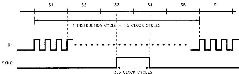
FIGURE 9-13. Instruction Cycle Timing
