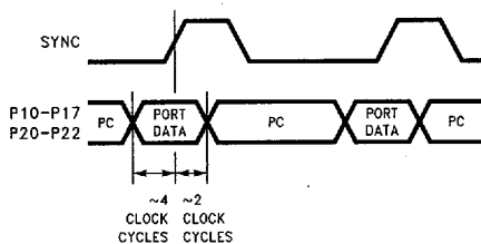
FIGURE 9-17. Timing Waveform of the PORT Lines in EA Mode
