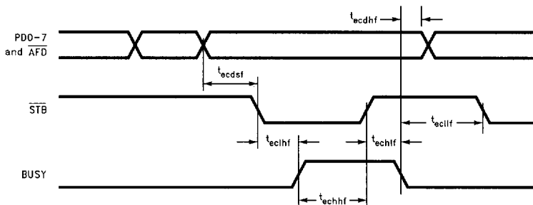
FIGURE 11-22. ECP Parallel Port Forward Timing Diagram
