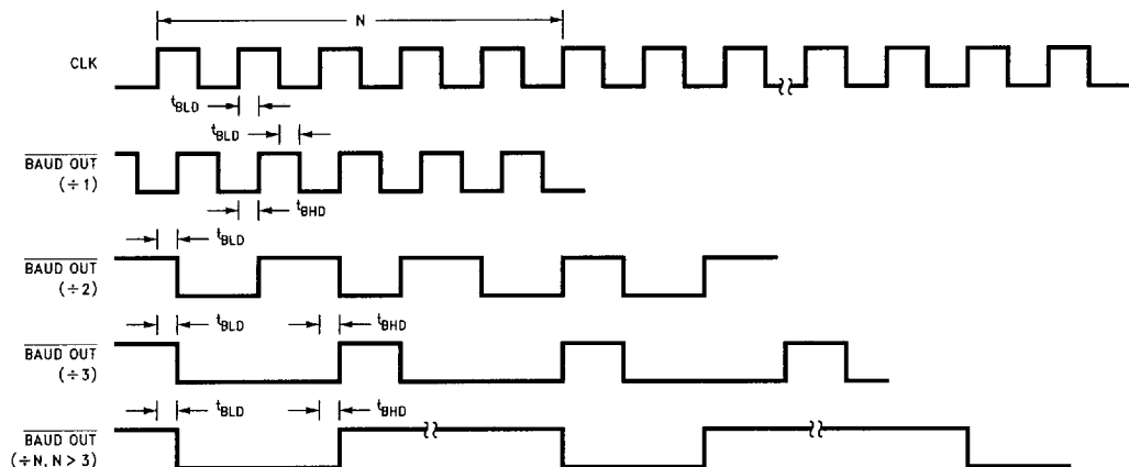
FIGURE 11-5. Baud Out Timing
