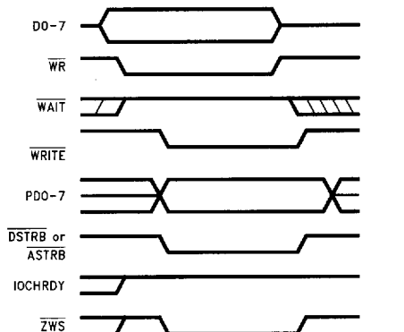
FIGURE 7-3. EPP Write with ZWS
