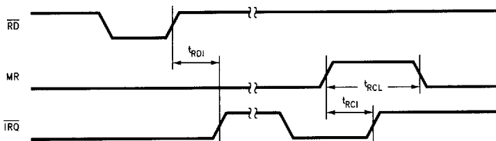
FIGURE 11-24. \overline{IRQ} Release Delay
