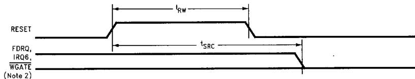
FIGURE 11-13. Reset Timing
