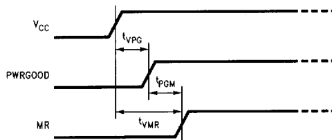
FIGURE 11-26. PWRGOOD MR Timing
