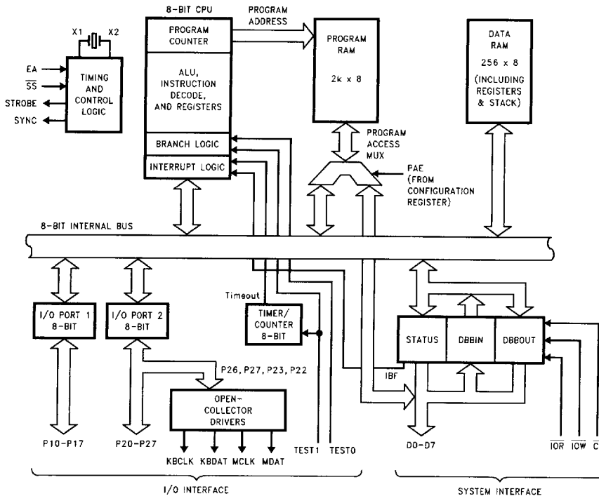
FIGURE 9-1. Keyboard Controller Functional Block Diagram
