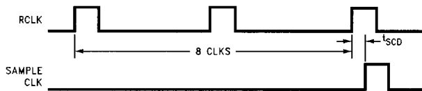
FIGURE 11-7. Sample Clock Timing
