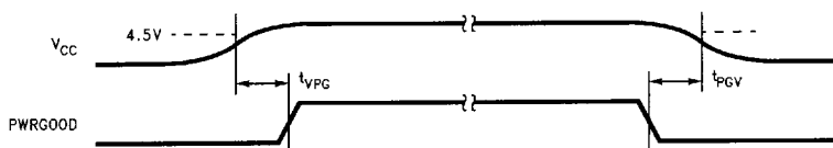
FIGURE 11-25. PWRGOOD V_{CC} Timing
