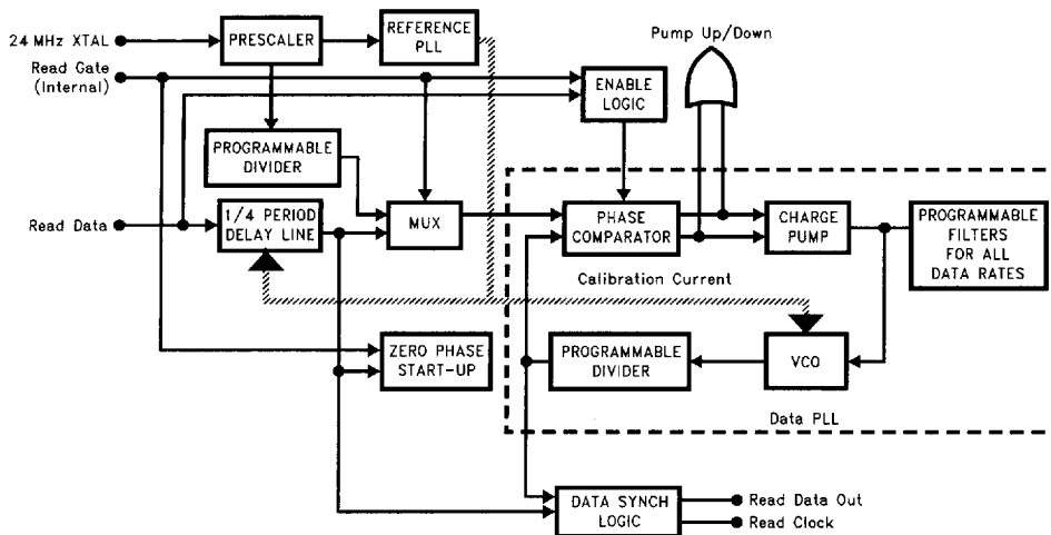
FIGURE 5-1. FDC Data Separator Block Diagram
