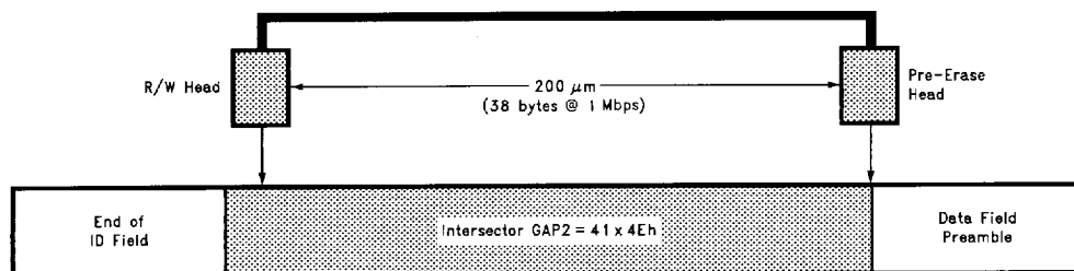
FIGURE 5-4. Perpendicular Recording Drive R/W Head and Pre-Erase Head
