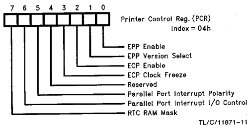
FIGURE 2-1. PC87323 Configuration Registers
