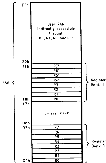
FIGURE 9-5. Keyboard Controller Data Memory Map
