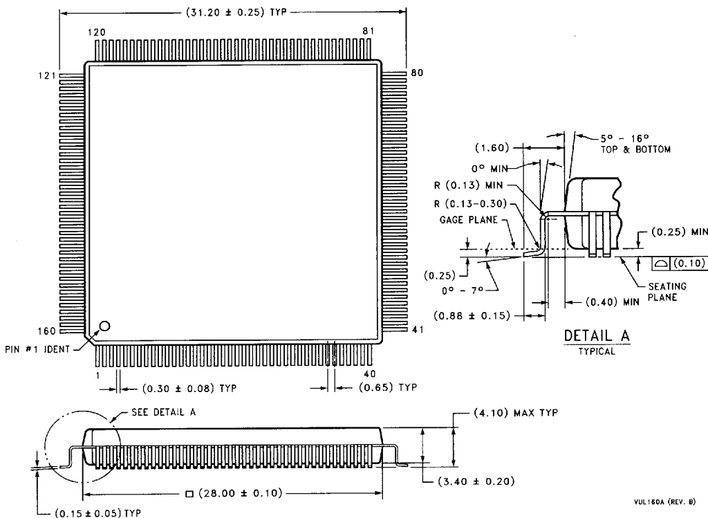
Plastic Quad Flatpak Order Number PC87323VUL NS Package Number VUL160A
