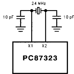
FIGURE 9-11. Internal Clock Connection
