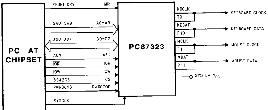
FIGURE 9-2. Keyboard Controller to Host System Interface
