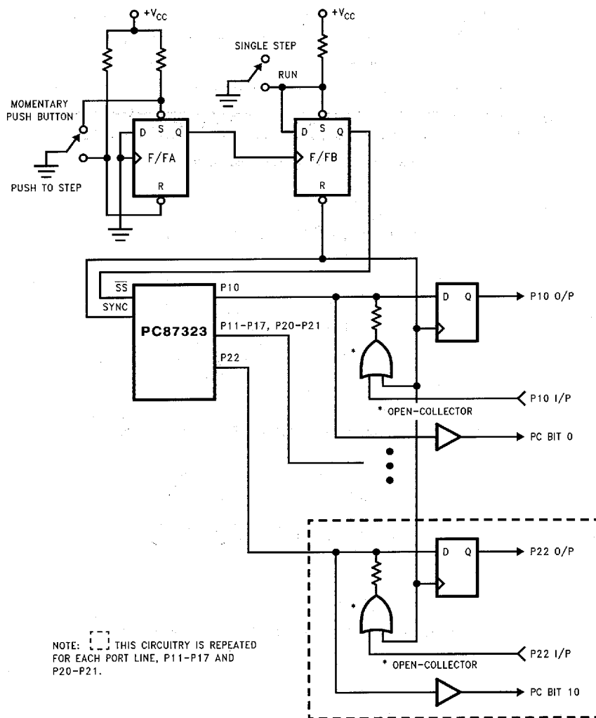
FIGURE 9-14. Example of Single-Step Circuit
