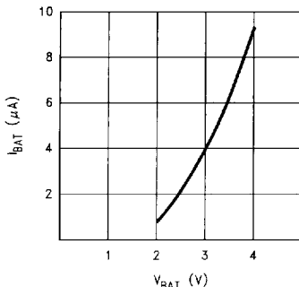
FIGURE 9-21. Typical Battery Current during Battery Backed Mode
