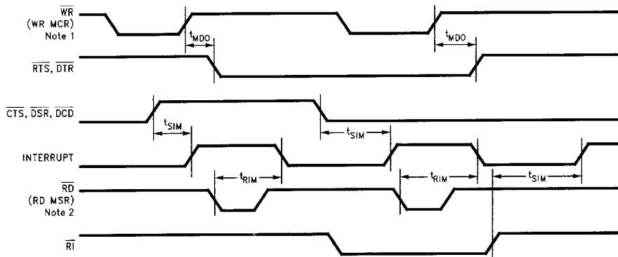
FIGURE 11-11. MODEM Control Timing
