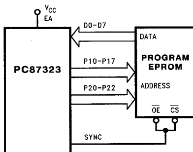
FIGURE 9-16. Connection of an External EPROM in EA Mode
