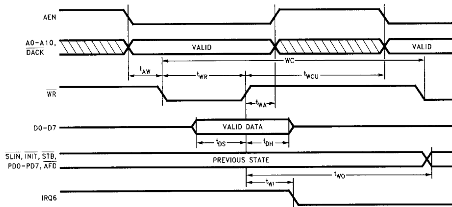
FIGURE 11-3. Microprocessor Write Timing
