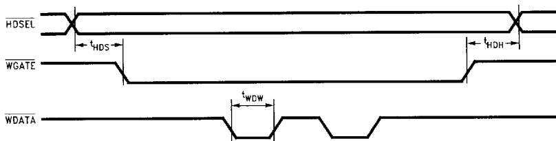
FIGURE 11-14. Write Data Timing
