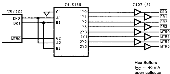
FIGURE 2-2. PC87323 Four Floppy Drive Circuit
