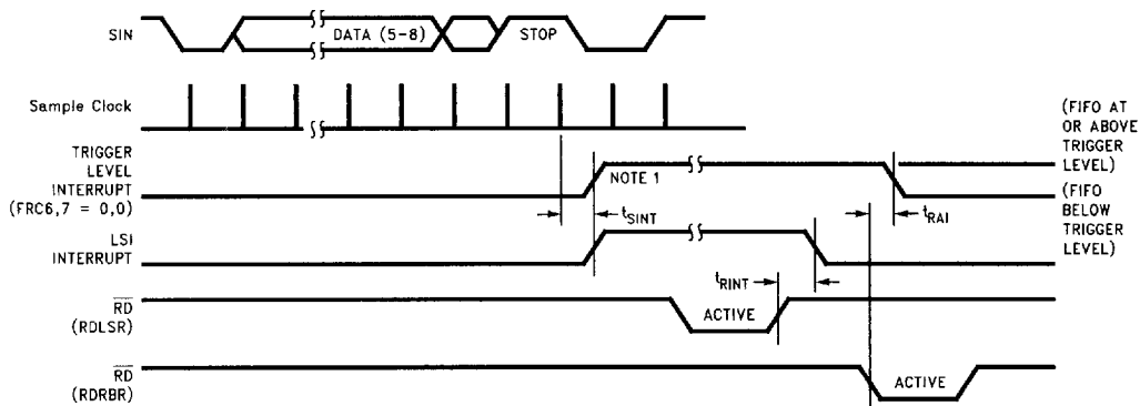
FIGURE 11-8. Receiver Timing
