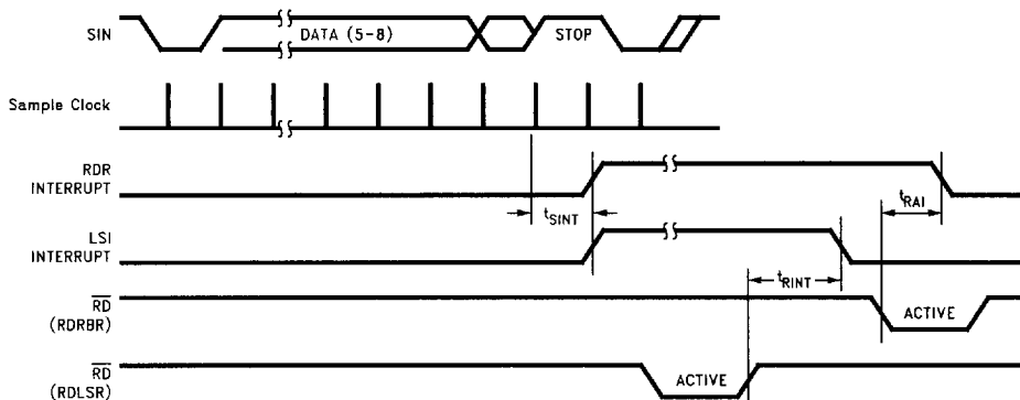
FIGURE 11-8. Receiver Timing
