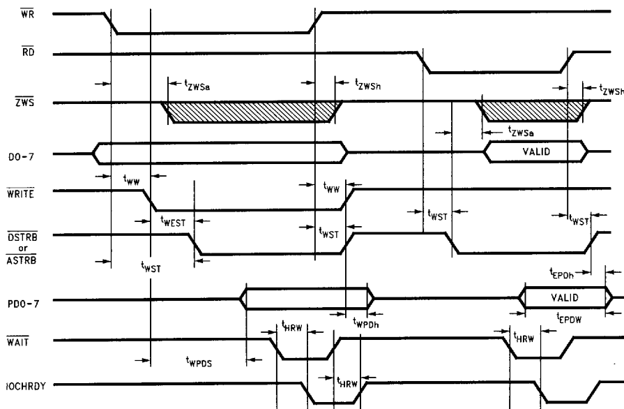
FIGURE 11-21. Enhanced Parallel Port Timing
