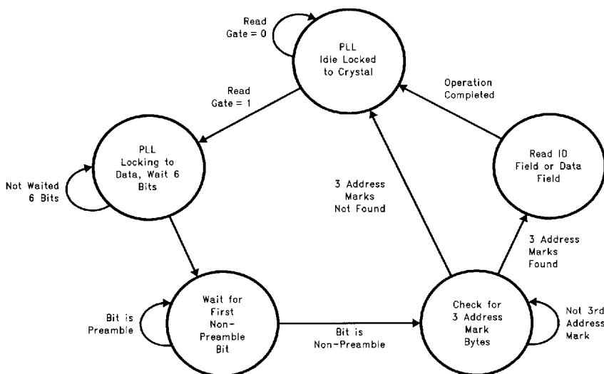
FIGURE 5-3. Read Data Algorithm—State Diagram
