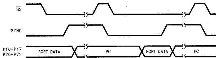
FIGURE 9-15. Single-Step Operation
