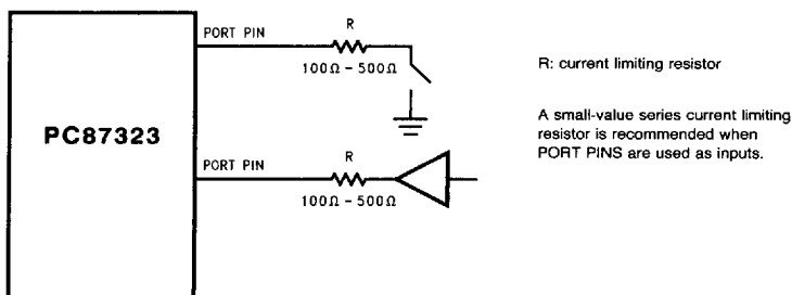
FIGURE 9-9. Using Port Pins as Inputs
