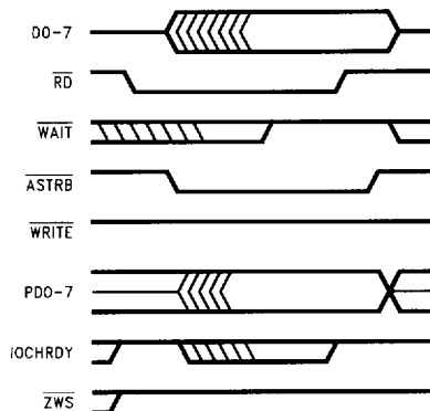
FIGURE 7-2. EPP 1.7 Address Read
