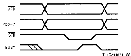
FIGURE 7-6. ECP Forward Write Cycle
