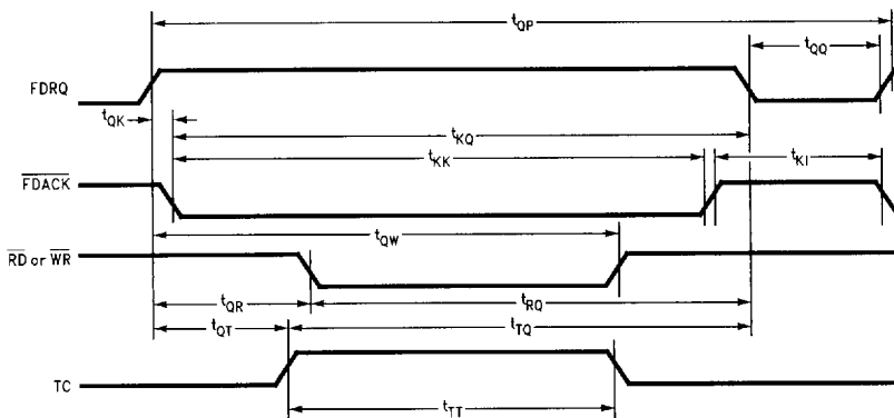
FIGURE 11-12a. FDC DMA Timing
