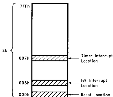
FIGURE 9-4. Keyboard Controller Program Memory Map
