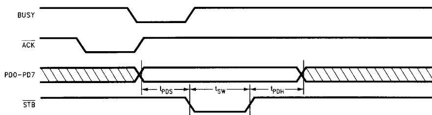
FIGURE 11-20. Typical Parallel Port Data Exchange
