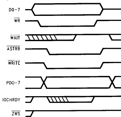
FIGURE 7-1. EPP 1.7 Address Write
