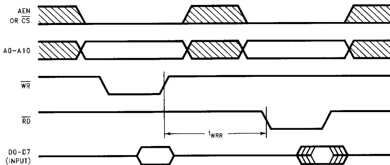
FIGURE 11-4. Read After Write Operation to All Registers and RAM Timing
