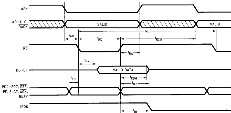
FIGURE 11-2. Microprocessor Read Timing
