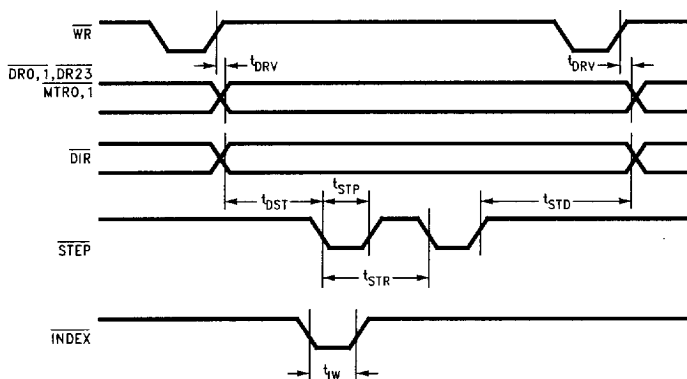
FIGURE 11-16. Drive Control Timing
