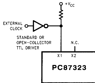
FIGURE 9-12. External Clock Connection
