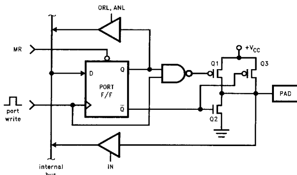
FIGURE 9-8. Active Pull-Up I/O Port Structure
