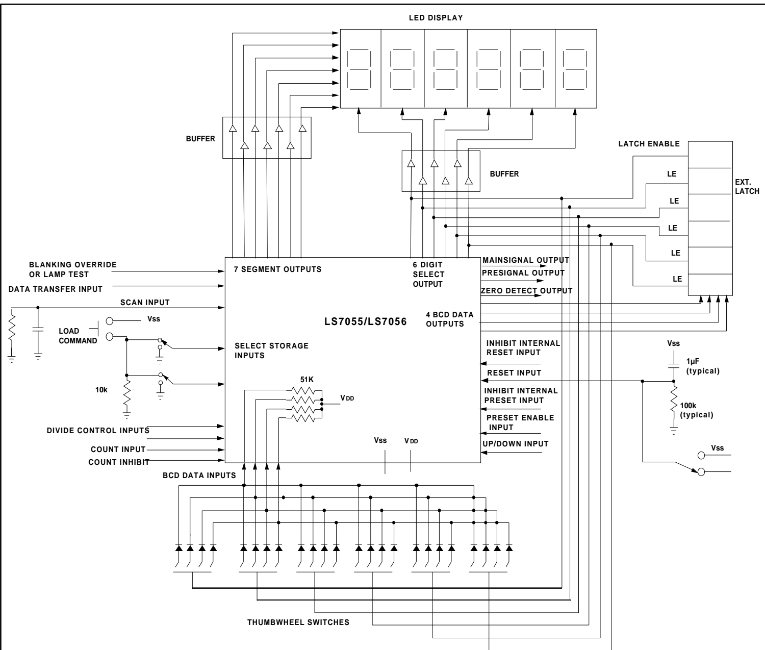
FIGURE 5. SYSTEM INTERCONNECTION DIAGRAM
