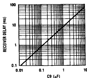
TL/H/7892-11 FIGURE 10. Receiver Delay vs C9
