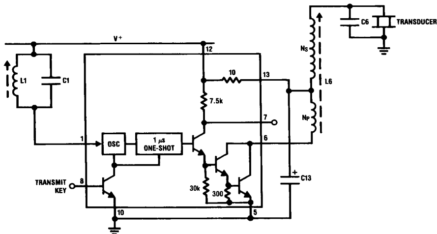
FIGURE 5. Transmitter
